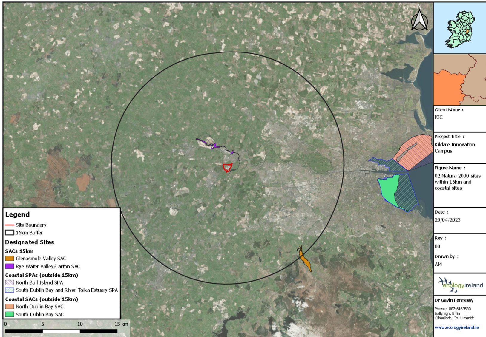
Figure 4-1 Designated Natura 2000 sites located in wider hinterland.
