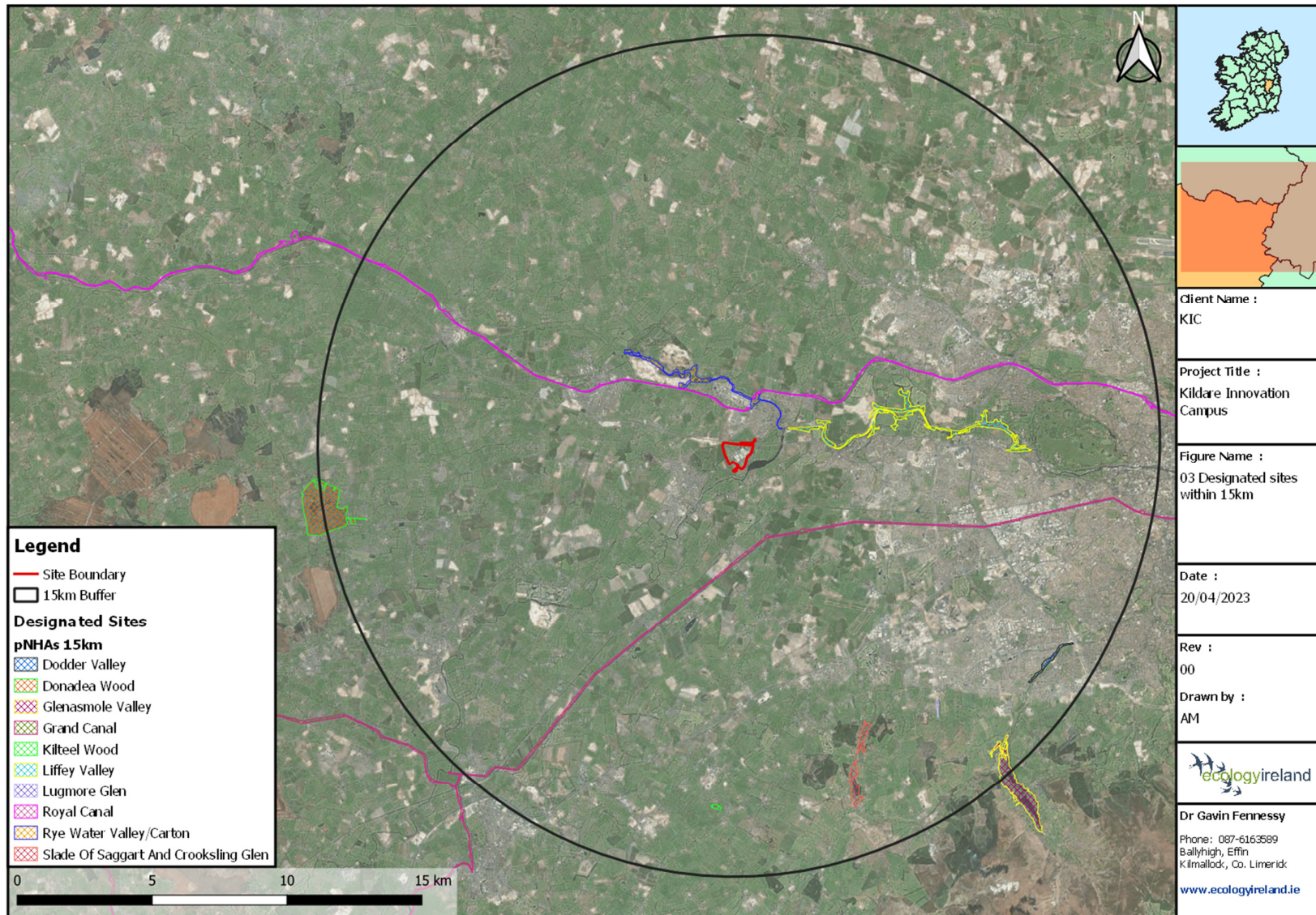
Figure 4-2 Nationally designated sites in wider hinterland.
