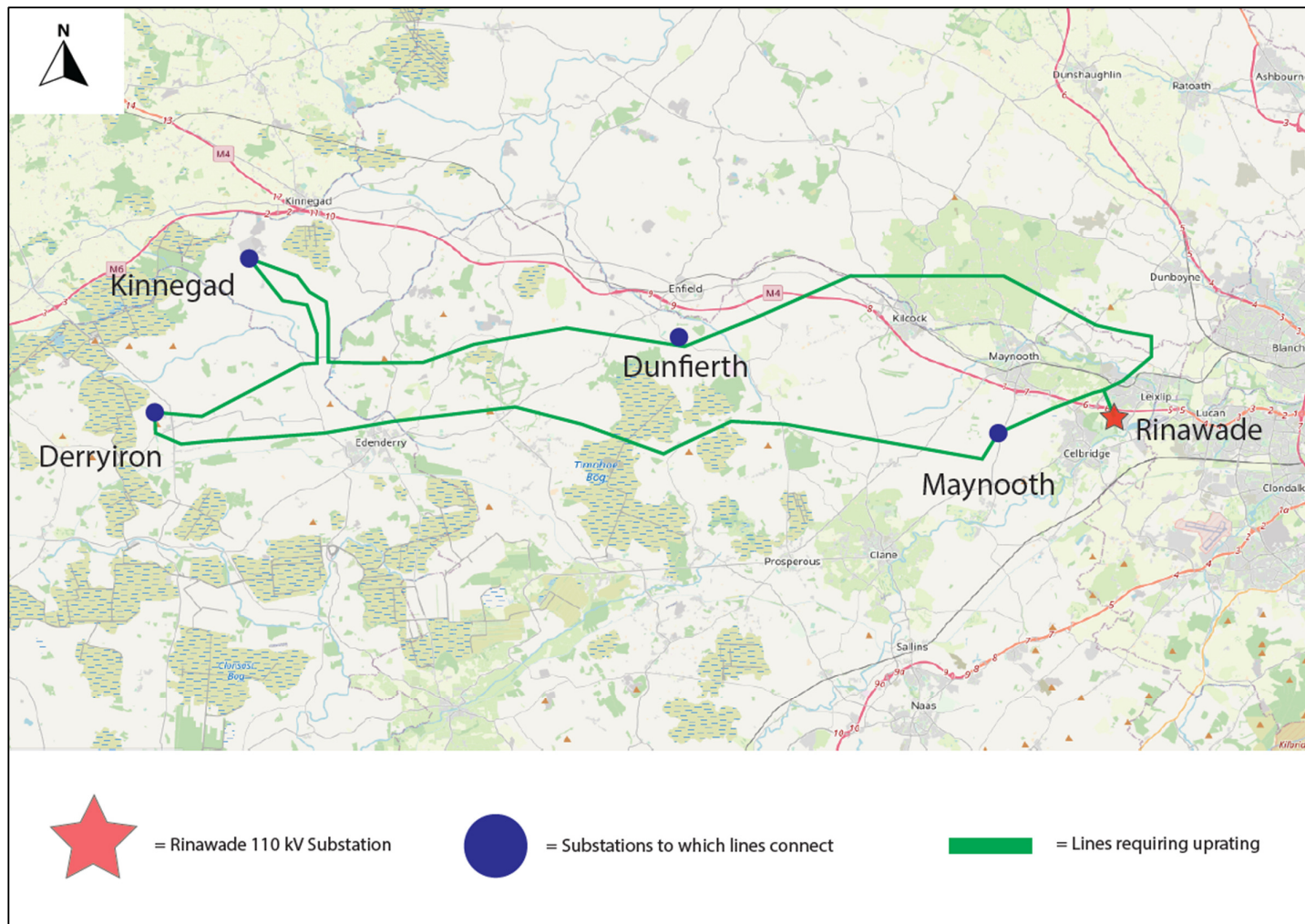
Figure 3-2 Existing 110kV routes requiring upgrading to facilitate the proposed development (from Chapter 2 of the Environmental Impact Assessment Report)
