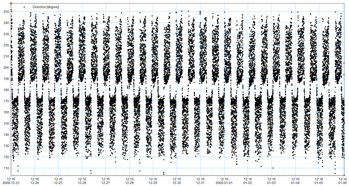
Figure 2-12 Full time series of current direction for current meter 1 (CM1)
