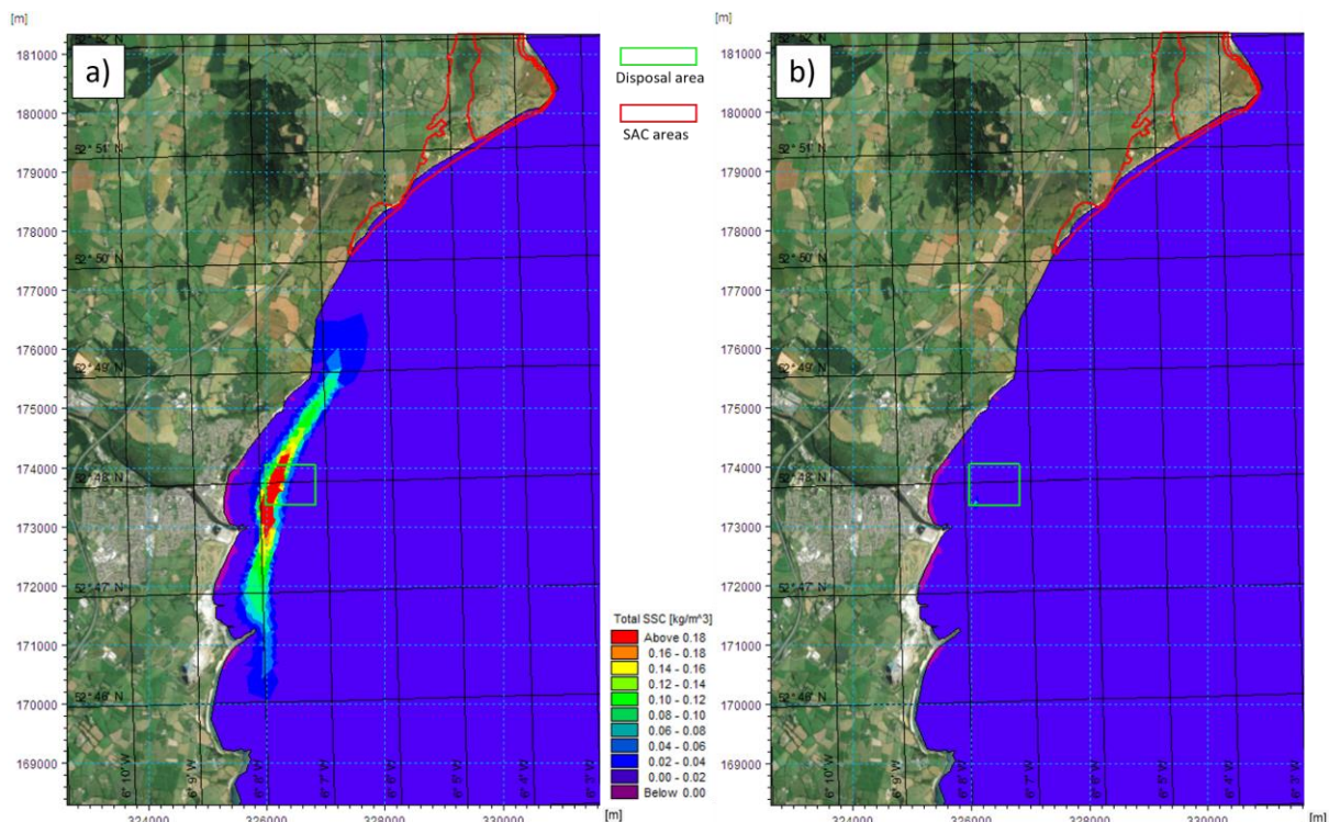
Figure 3-9 Fraction 3 SSC – close-up view - considering the 18-day simulation: (a) maximum values and (b) mean values.
