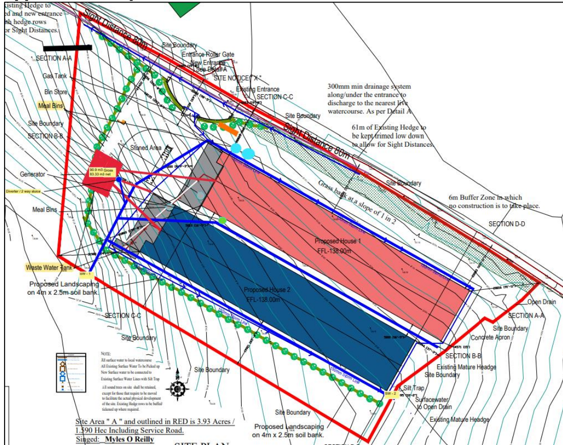
Excerpt from Drawing No. P02, titled "Site Plan" received by the Agency in support of the application on 19 August 2023.
