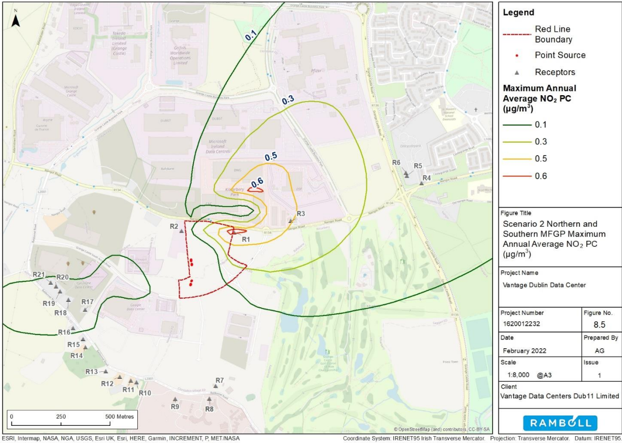
Figure 8.5 Scenario 2 Northern and Southern MFGP Maximum Annual Average NO 2 PC (µg/m 3 ).
