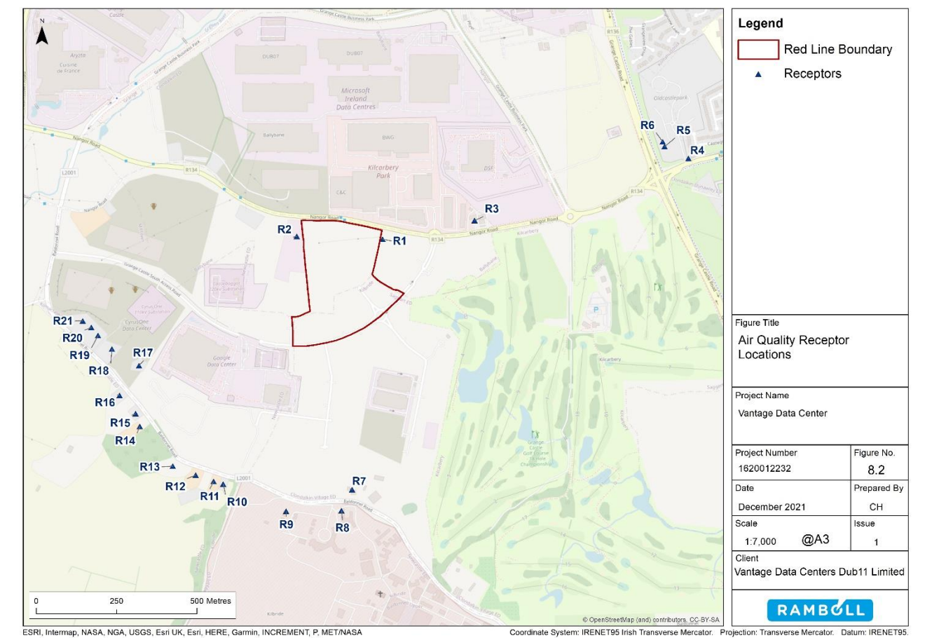
Figure 8.2: Air Quality Receptor Locations
