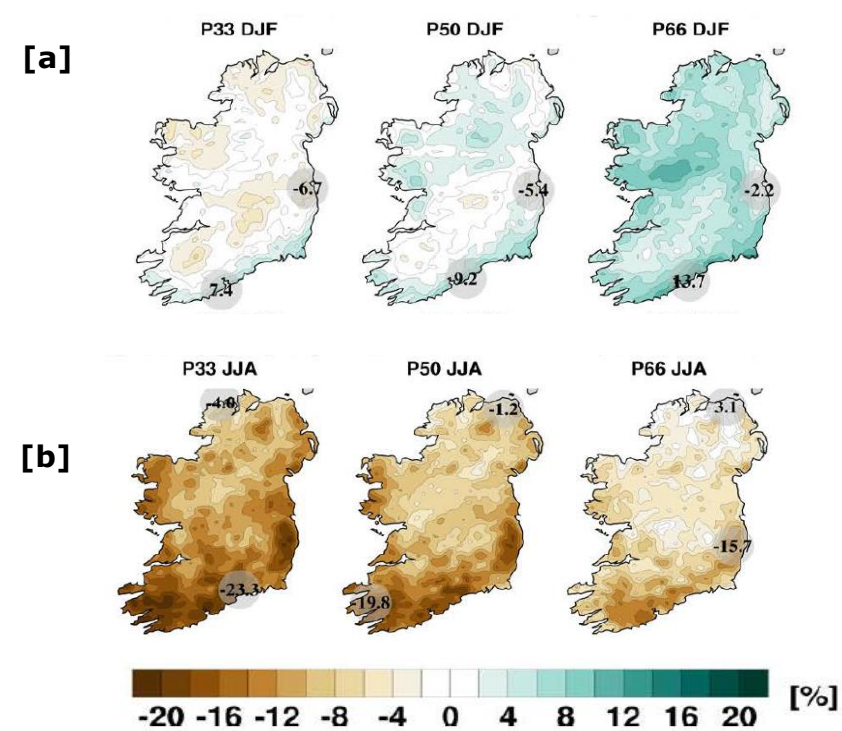
Figure 13-2 The 33rd, 50th and 66th percentiles of [a] winter and [b] summer mean precipitation projections for the RCP 8.5 scenario. The future period (2041-2060) is compared with the reference period (1981-2000). The numbers on each plot are the minimum and maximum projected changes at their locations
