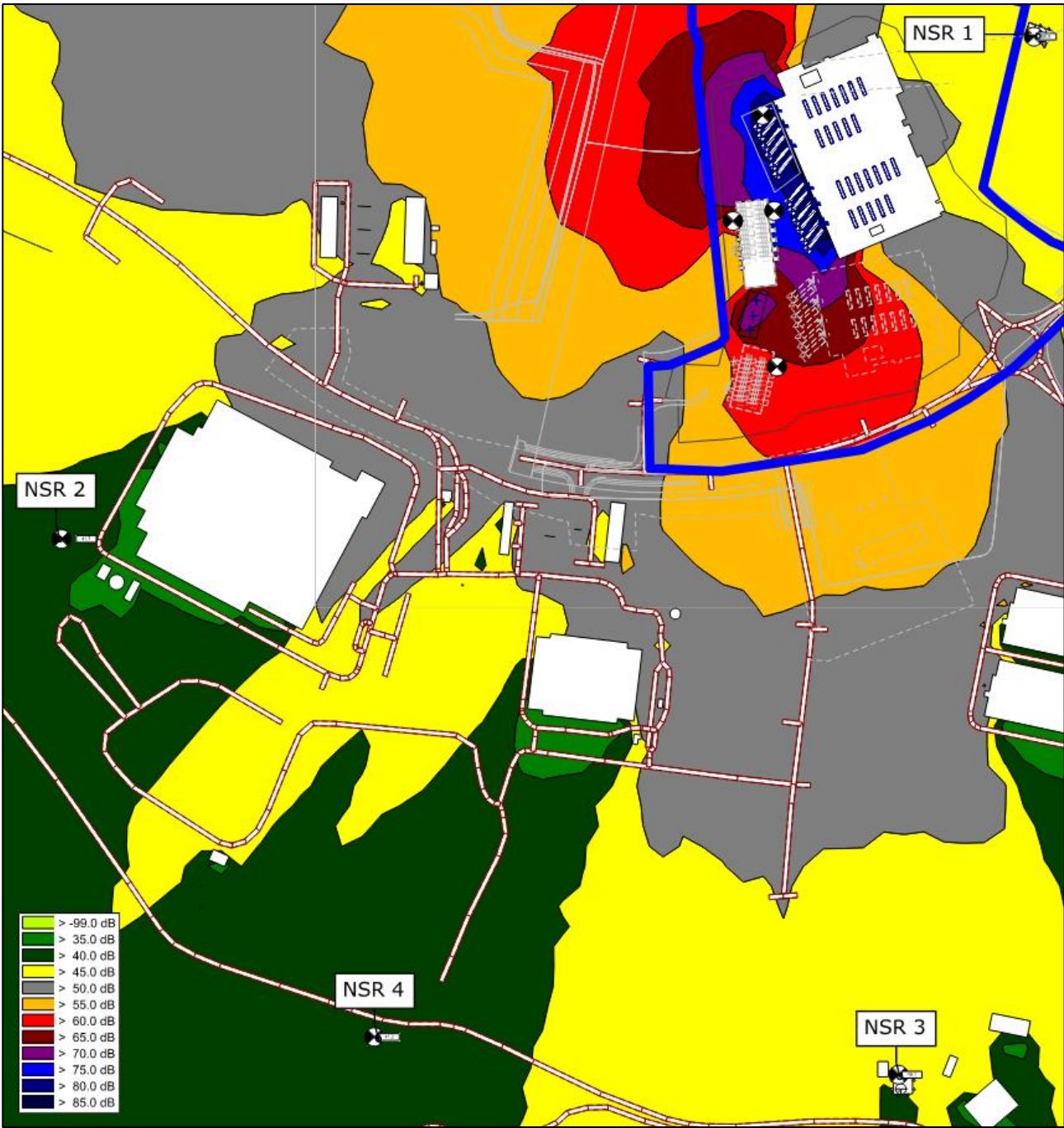
Figure 9.8: Overview of modelled emergency noise emissions (Scenario 1) Grid set at 4.0 AGL
