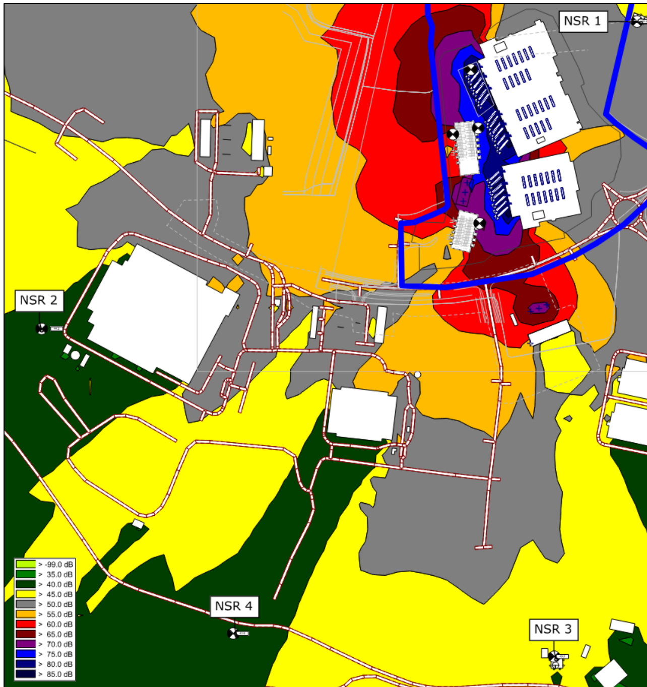
Figure 9.9: Overview of modelled emergency noise emissions (Scenario 2) Grid set at 4.0 AGL
