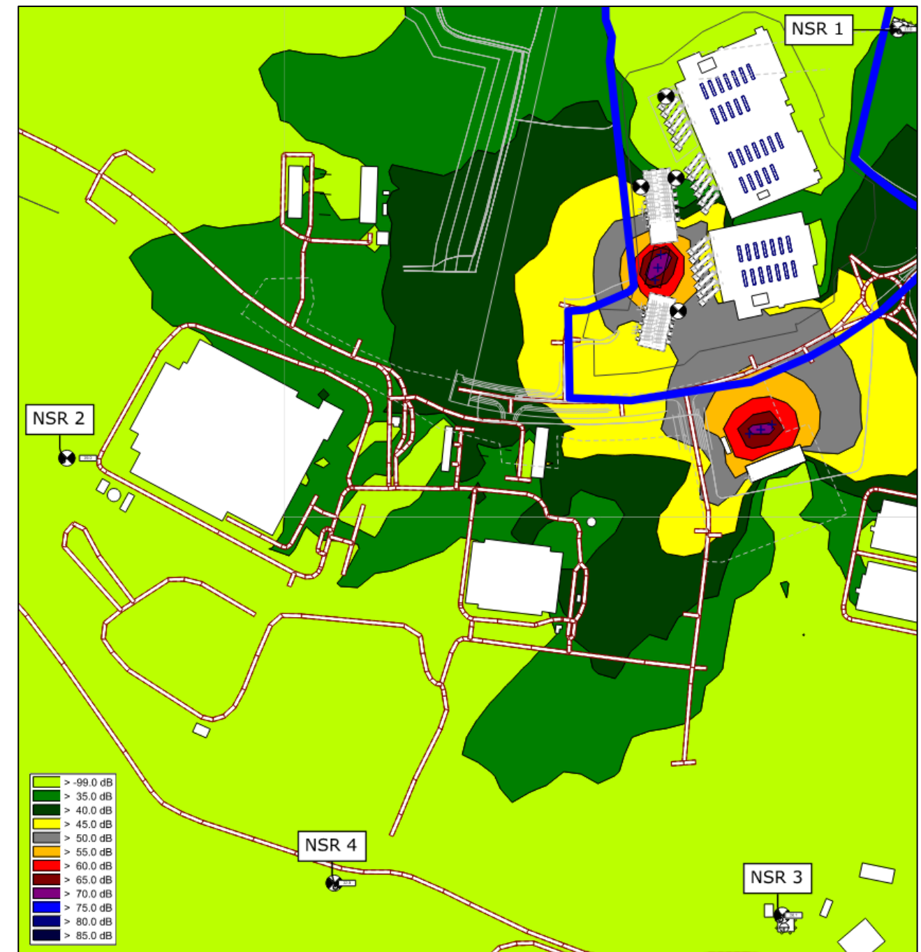
Figure 9.8: Overview of modelled noise emissions (Scenario 3) Grid set at 4.0 AGL
