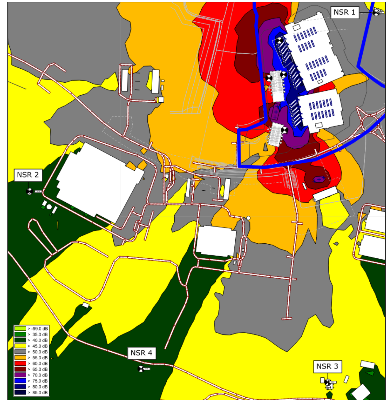
Figure 9.10: Overview of modelled emergency noise emissions (Scenario 3) Grid set at 4.0 AGL
