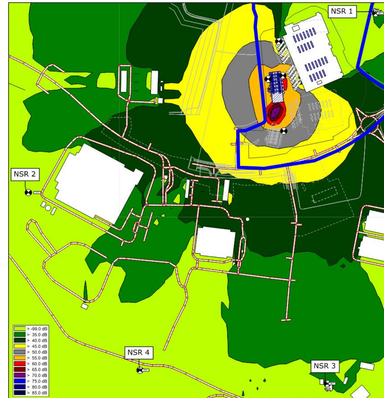
Figure 9.6: Overview of modelled noise emissions (Scenario 1) Grid set at 4.0 AGL
