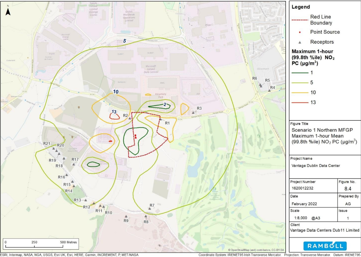
Figure 8.4: Phase 1 Northern MFGP Maximum 1-hour mean (99.8 th percentile) NO 2 PC (µg/m 3 ).
