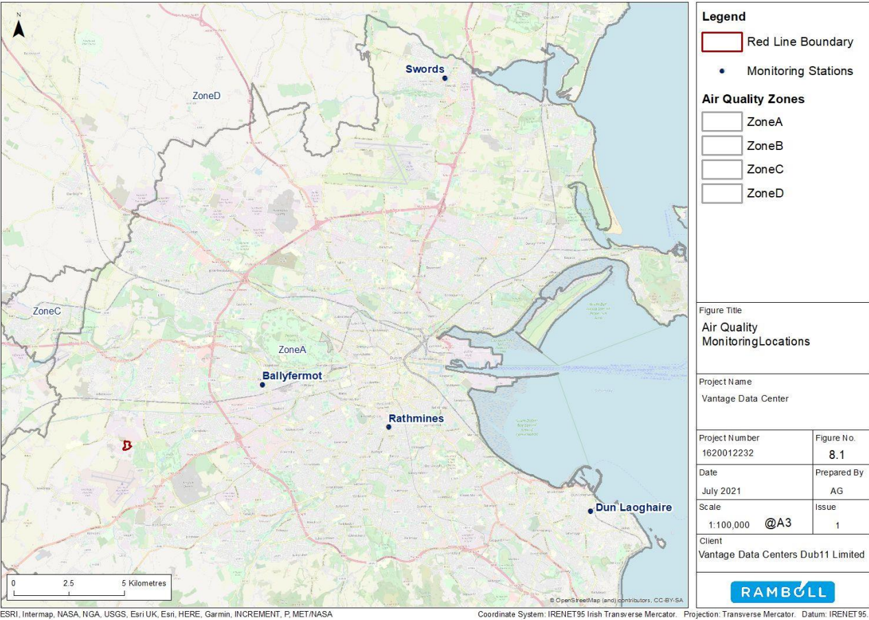
Figure 8.1: Air Quality Monitoring Locations
