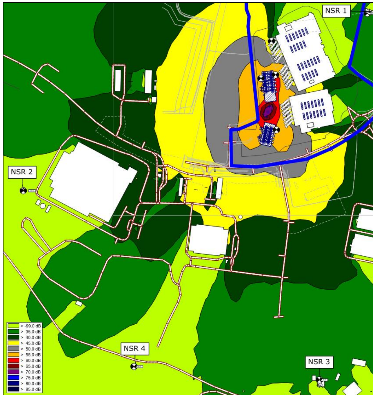
Figure 9.7: Overview of modelled noise emissions (Scenario 2) Grid set at 4.0 AGL
