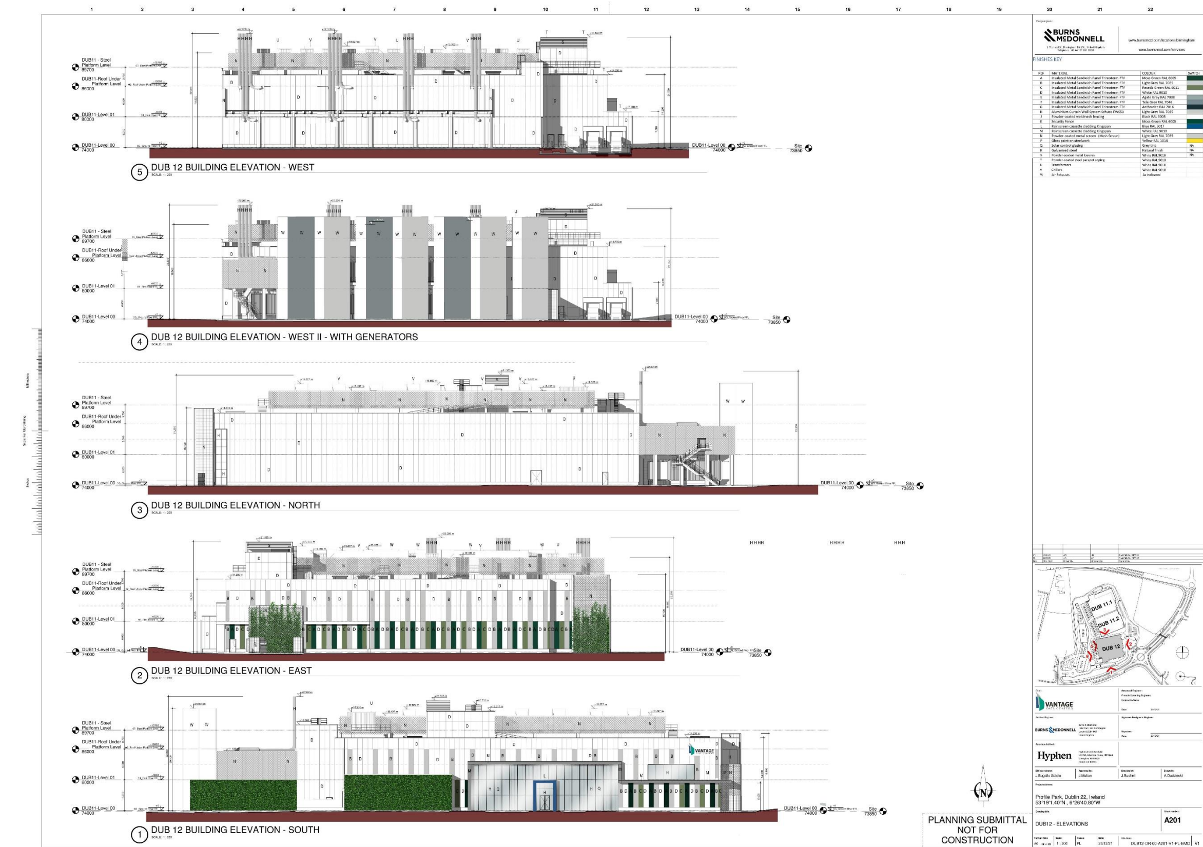
Figure 4.4: DUB12 Elevations (Source Burns & McDonnell)
