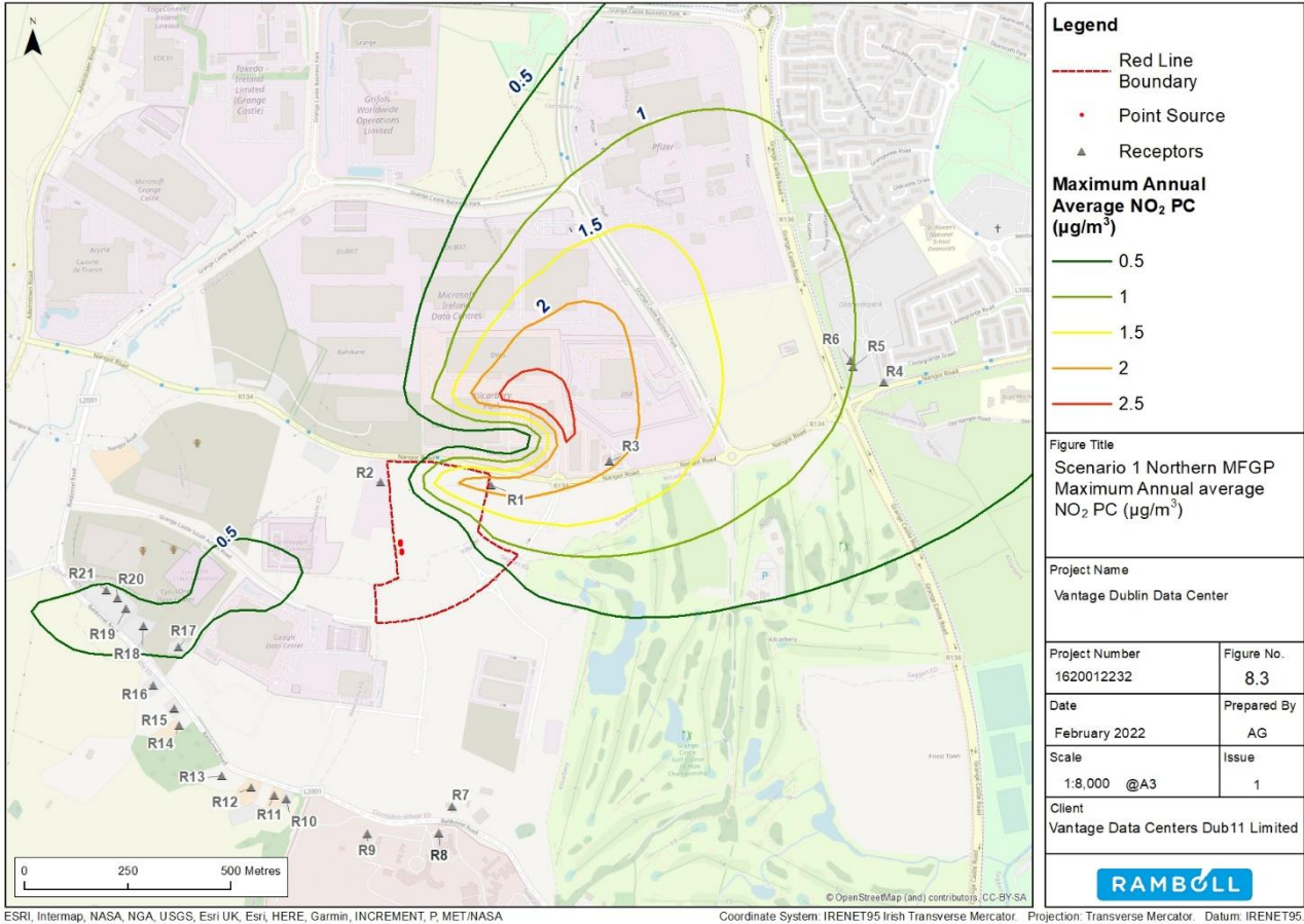
Figure 8.3: Scenario 1 Northern MFGP Maximum Annual Average NO 2 PC (µg/m 3 ).
