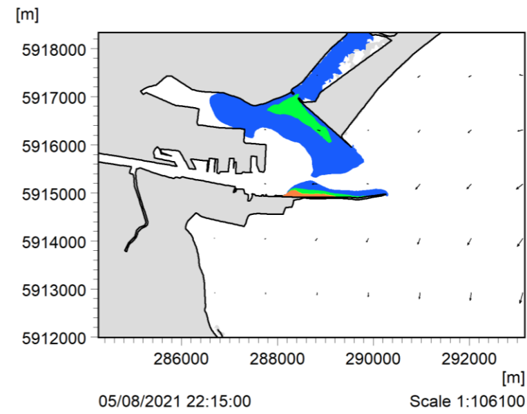
MRP 6 Mass Emissions – Summer Subsequent LW 2 days and 6 hours after the end of the mass emissions discharge.
