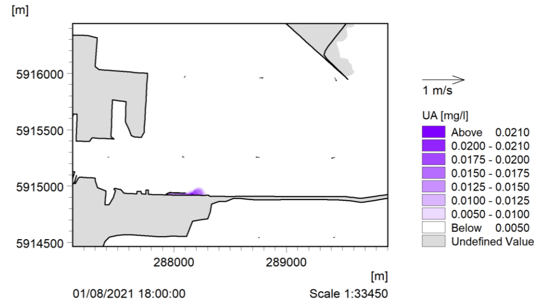
UA 1 Mass Emissions – Summer HW coinciding with the end of the mass emissions discharge.
