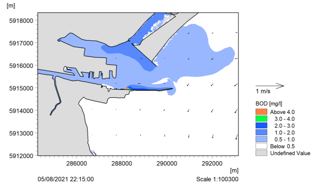
BOD 6 Mass Emissions – Summer Subsequent LW 2 days and 6 hours after the end of the mass emissions discharge.
