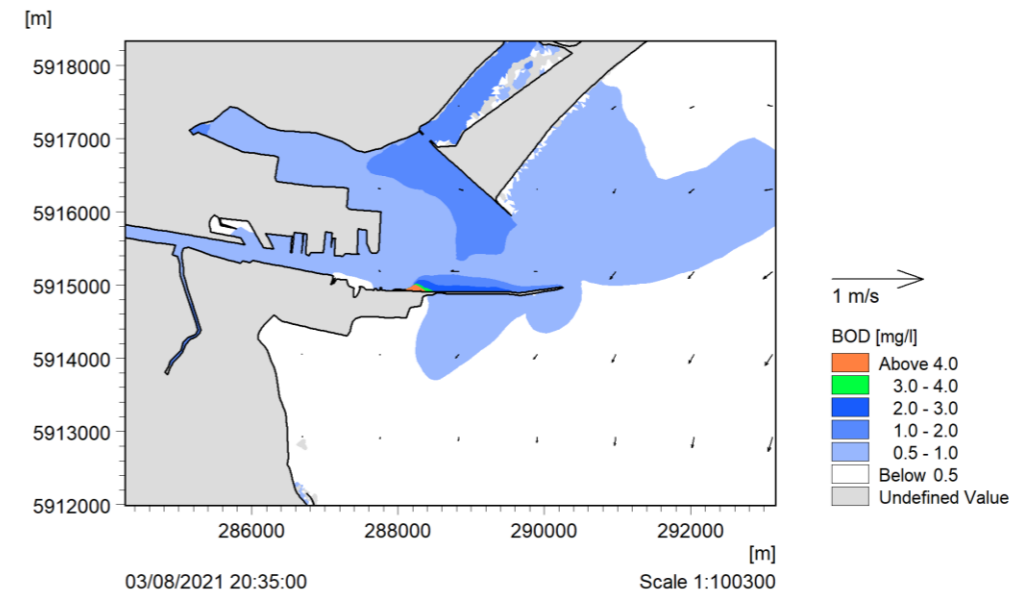
BOD 5 Mass Emissions – Summer HW, 2 days after the end of the mass emissions discharge.
