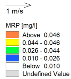
MRP 6 Mass Emissions – Summer Subsequent LW 2 days and 6 hours after the end of the mass emissions discharge.
