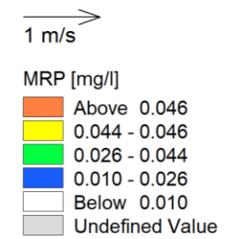
MRP 7 Mass Emissions – Summer HW, 4 days after the end of the mass emissions discharge.
