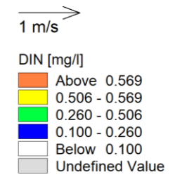
DIN 1 Mass Emissions – Summer HW coinciding with the end of the mass emissions discharge.
