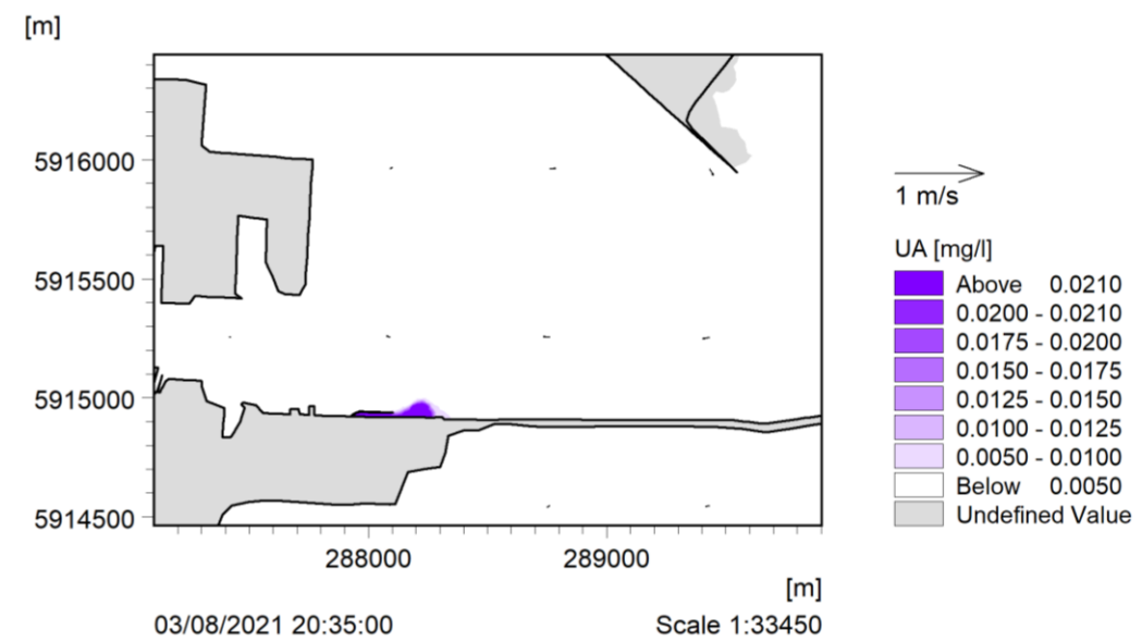
UA 5 Mass Emissions – Summer HW, 2 days after the end of the mass emissions discharge.
