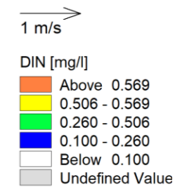
DIN 5 Mass Emissions – Summer HW, 2 days after the end of the mass emissions discharge.
