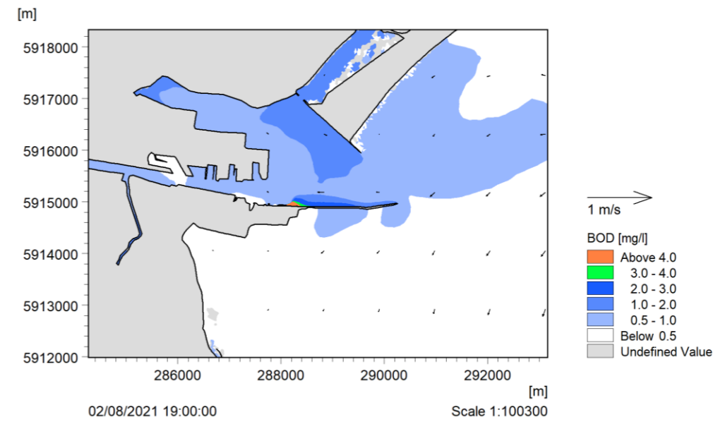
BOD 3 Mass Emissions – Summer HW, 1 day after the end of the mass emissions discharge.
