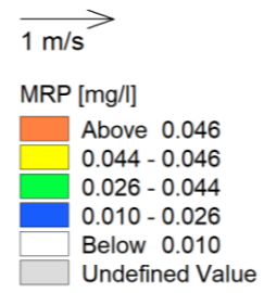
MRP 8 Mass Emissions – Summer Subsequent LW 4 days and 6 hours after the end of the mass emissions discharge.
