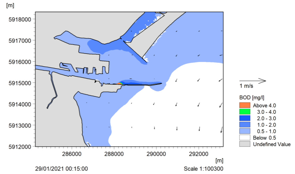
BOD 6 Mass Emissions – Winter Subsequent LW 2 days and 6 hours after the end of the mass emissions discharge.
