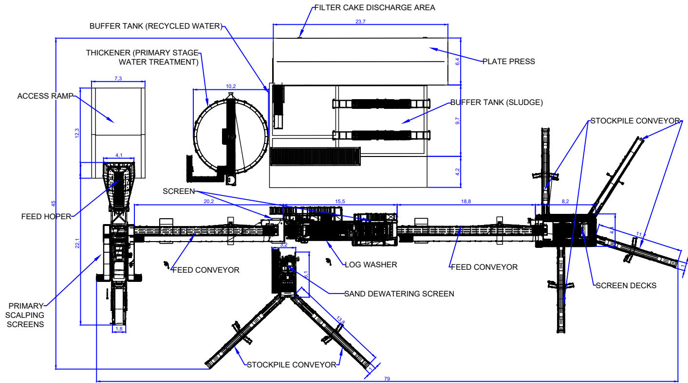
PLAN LAYOUT
