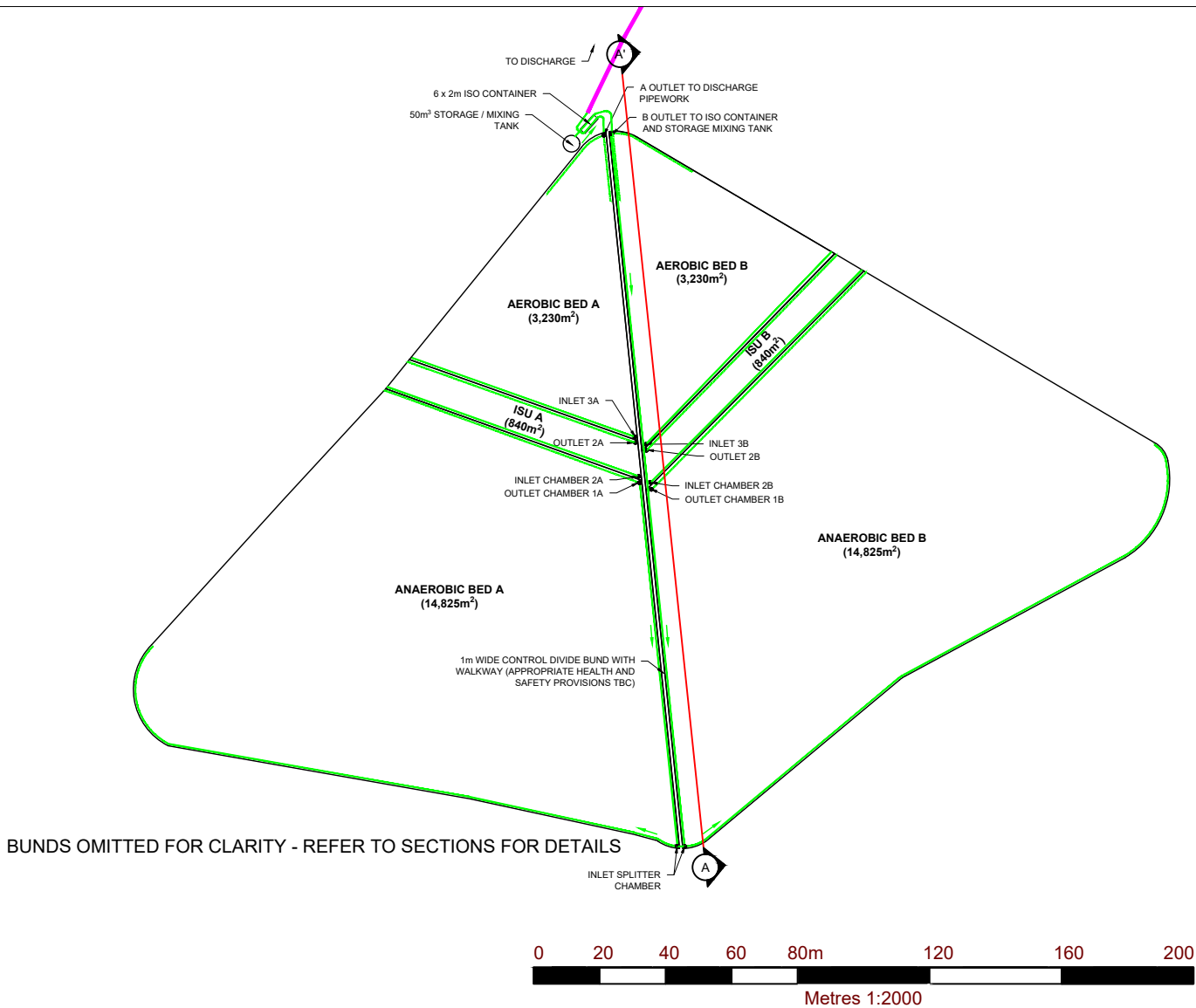
INDICATIVE PROPOSED TREATMENT LAYOUT - PLAN VIEW SCALE 1:2000
