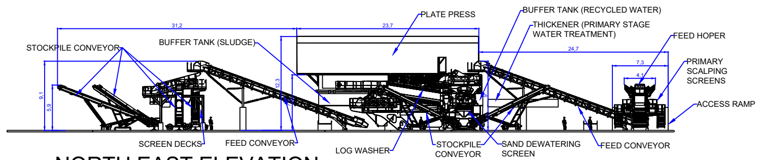
NORTH EAST ELEVATION
