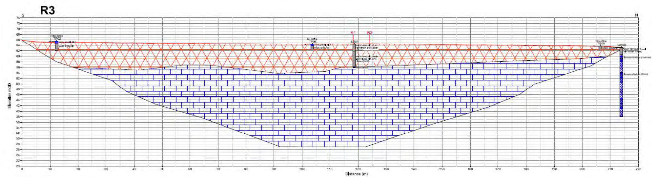
Figure 3-5: ERT Profile R3 Interpreted Cross Section
