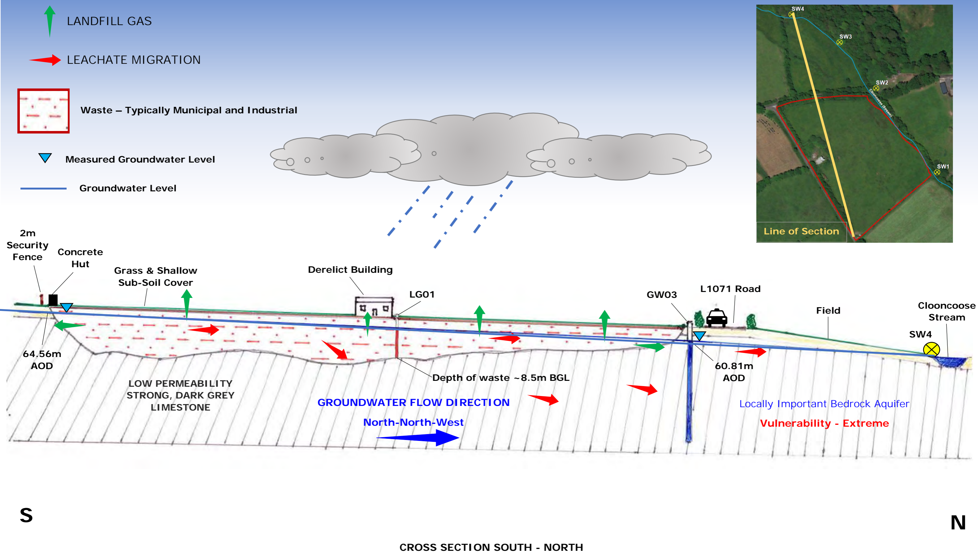
FIGURE 5.1 CARTRON BIG HISTORIC LANDFILL CONCEPTUAL SITE MODEL
