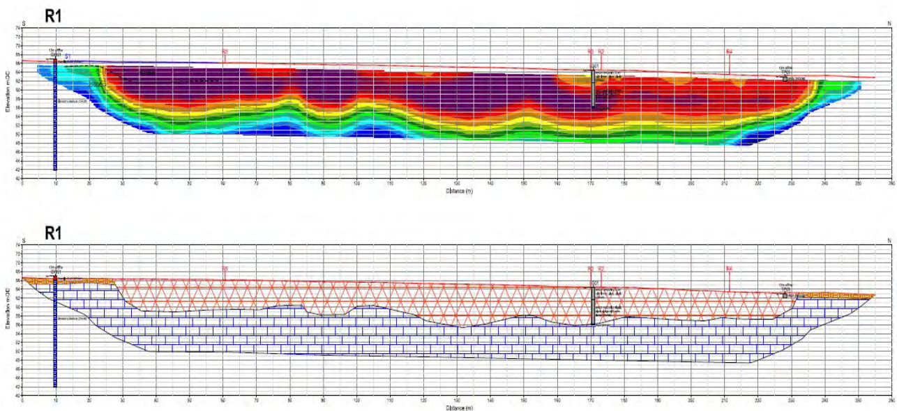
Figure 3-3: ERT Profile R1 Interpreted Cross Section
