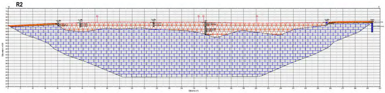
Figure 3-4: ERT Profile R2 Interpreted Cross Section
