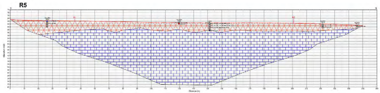
Figure 3-7: ERT Profile R5 Interpreted Cross Section
