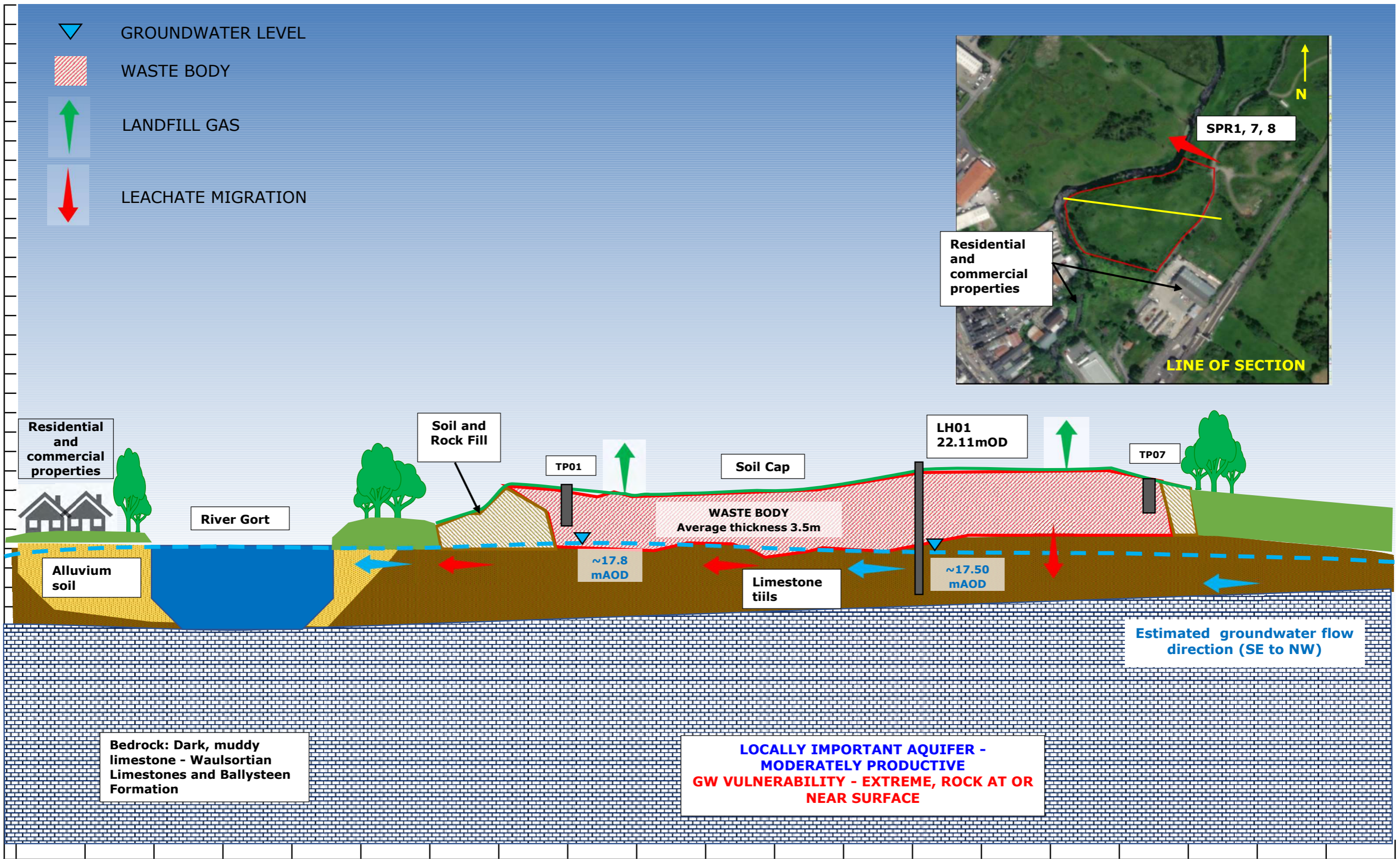
FIGURE 2.1 GORT HISTORIC LANDFILL CONCEPTUAL SITE MODEL
