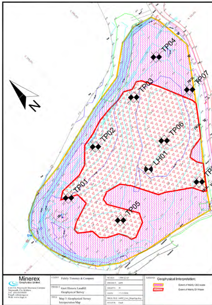
Figure 3-4: Geophysical Survey Estimated Waste Footprint
