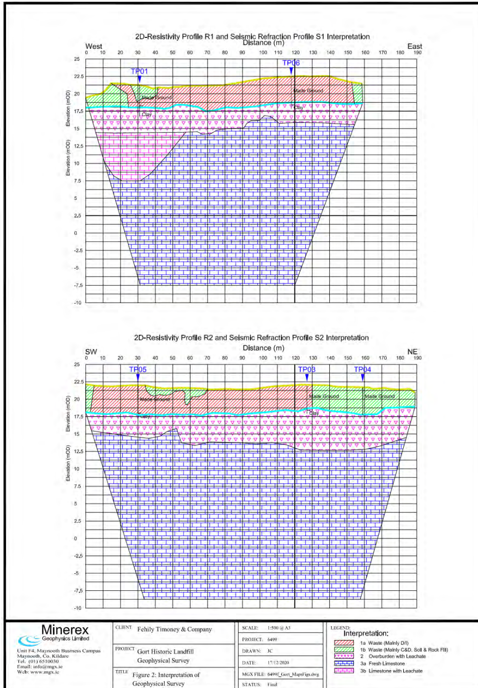
Figure 3-3: Integration of Geophysical Survey
