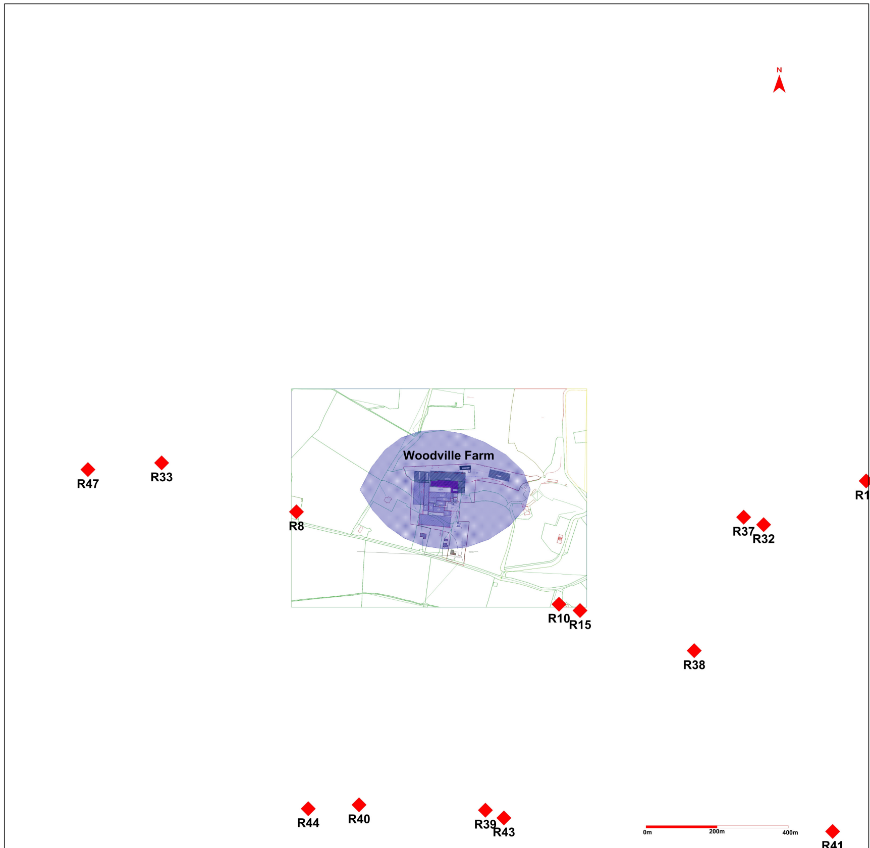
Figure 7.7. Predicted Ammonia plume spread of the proposed pig production facility for the Annual averages Ammonia concentrations of \leq 3.0 \mu\text{g}/\text{m}^3 yr 2017 ( — ).
