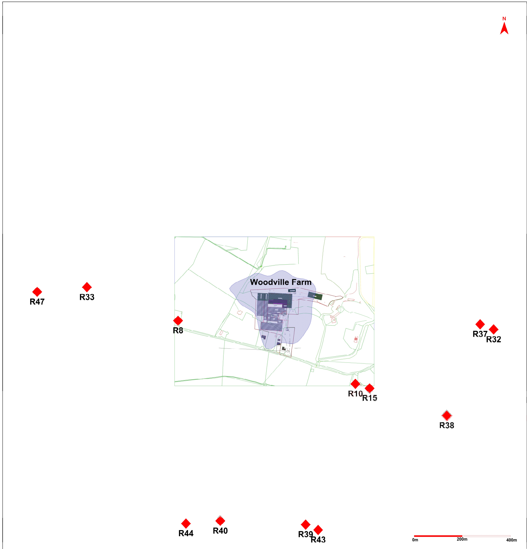
Figure 7.2. Predicted odour plume spread of the existing pig production facility for at the 98 th percentile of hourly averages for an odour concentrations of \leq 6.0 \text{ Ou}_E/\text{m}^3 \text{ yr 2017} ( — ).
