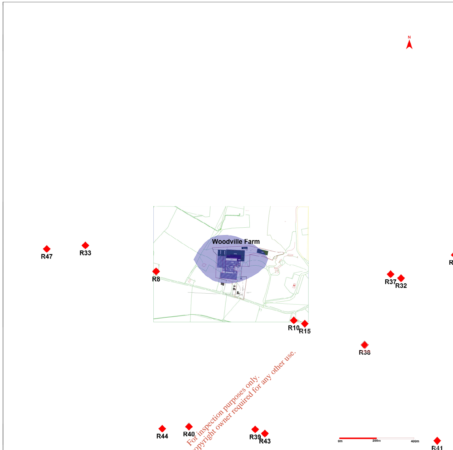
Figure 7.7. Predicted Ammonia plume spread of the proposed pig fattening facility for the Annual averages Ammonia concentrations of \leq 3.0 \mu\text{g}/\text{m}^3 \text{ yr} 2017 (■).
