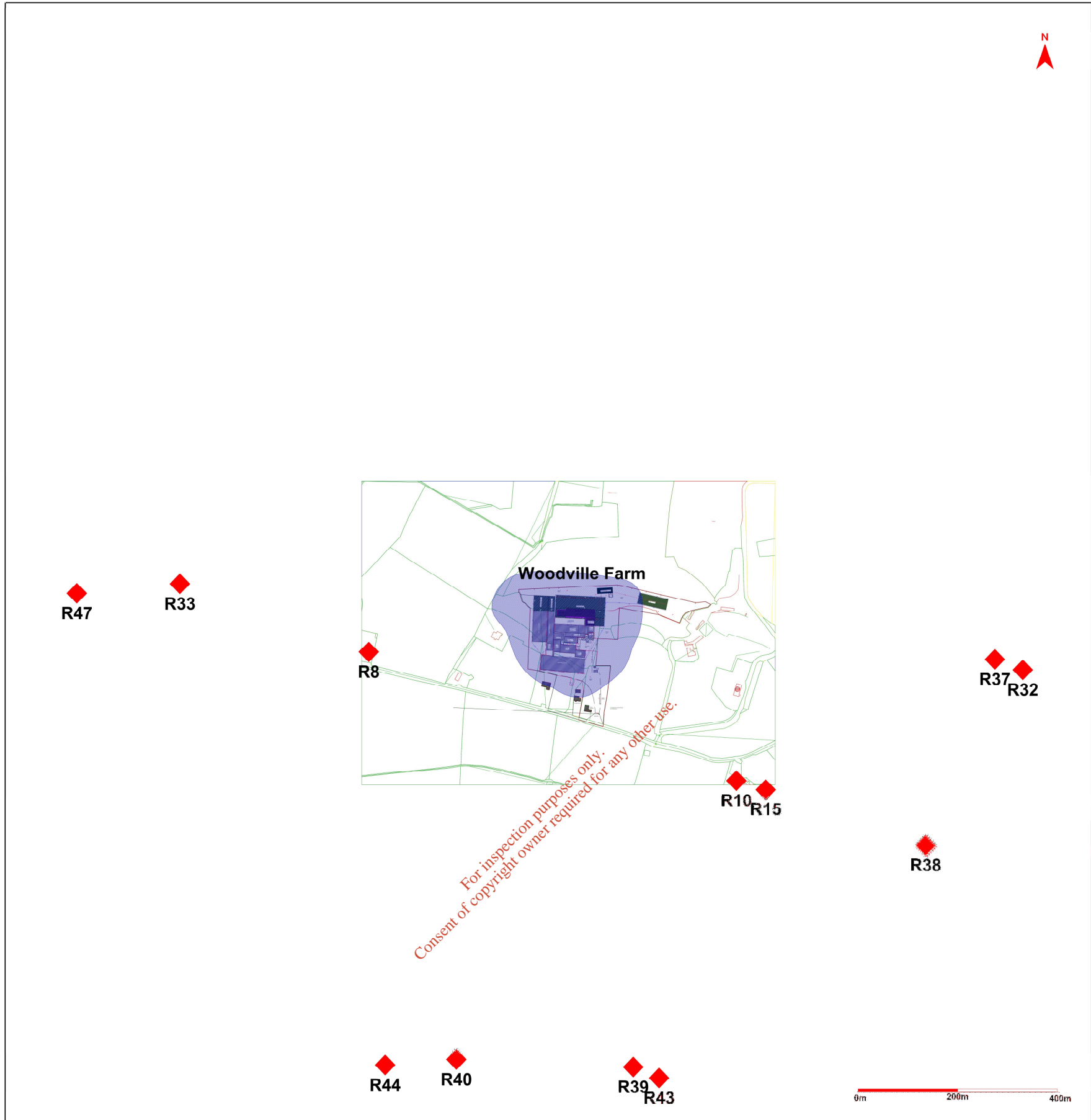
Figure 7.5. Predicted Ammonia plume spread of the existing pig fattening facility for the Annual averages Ammonia concentrations of \leq 3.0 \mu\text{g}/\text{m}^3 yr 2017 (■).
