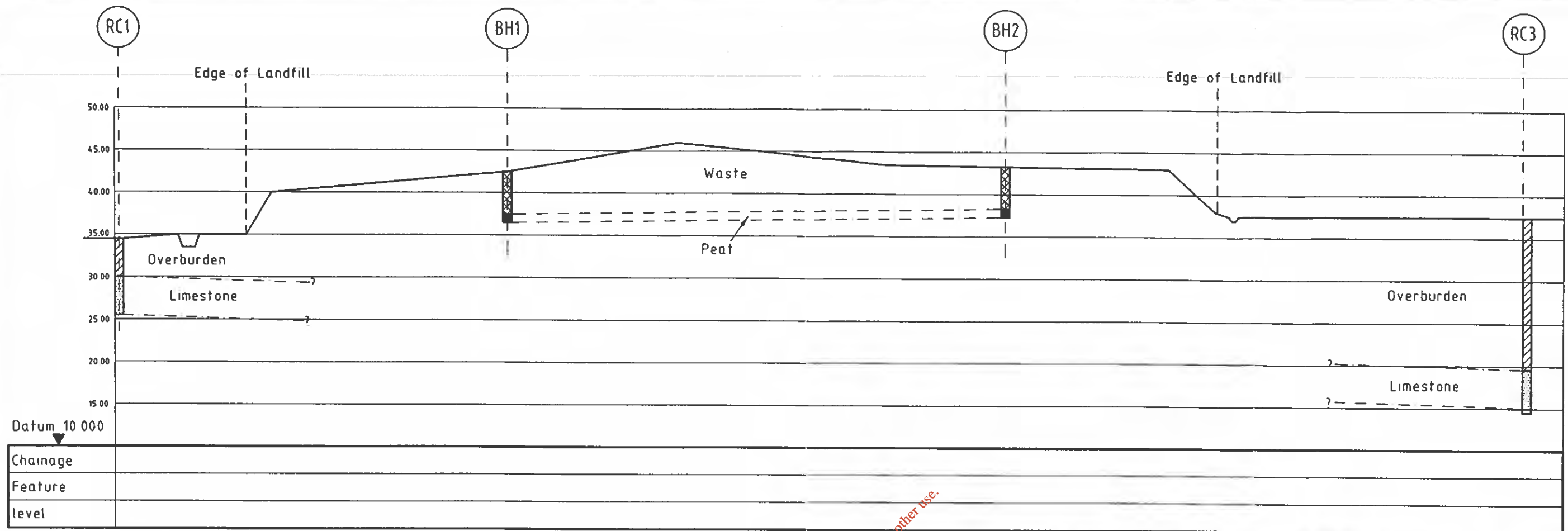
SECTION A-A SCALE 1:1000 HOR 1:500 VER
