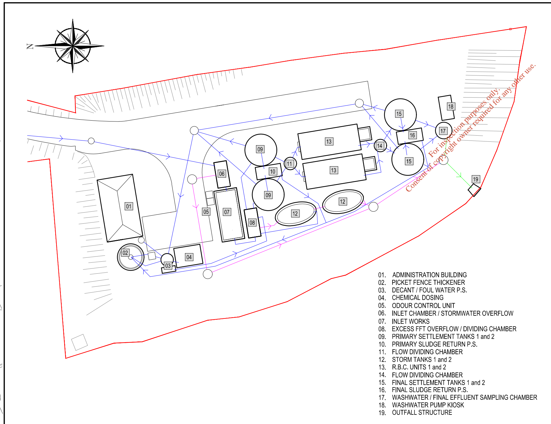
WASTE WATER TREATMENT PLANT - SITE LAYOUT PLAN SCALE 1:333
