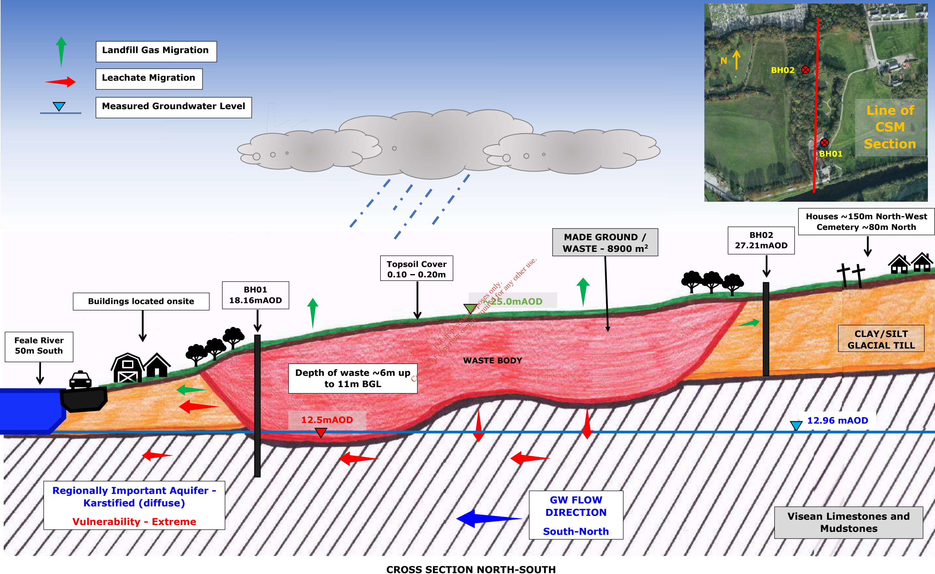
FIGURE 5.1 Listowel HISTORIC LANDFILL CONCEPTUAL SITE MODEL
