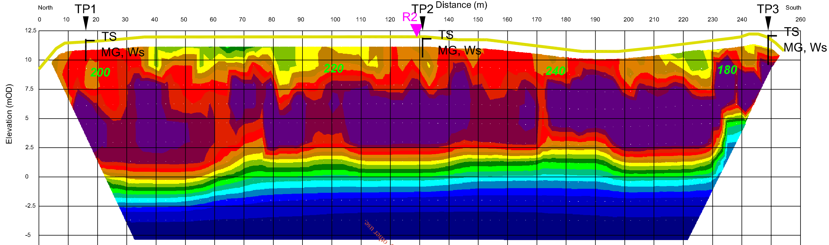
2D-Resistivity Profile R2 and Seismic Refraction Profile S2 Model
