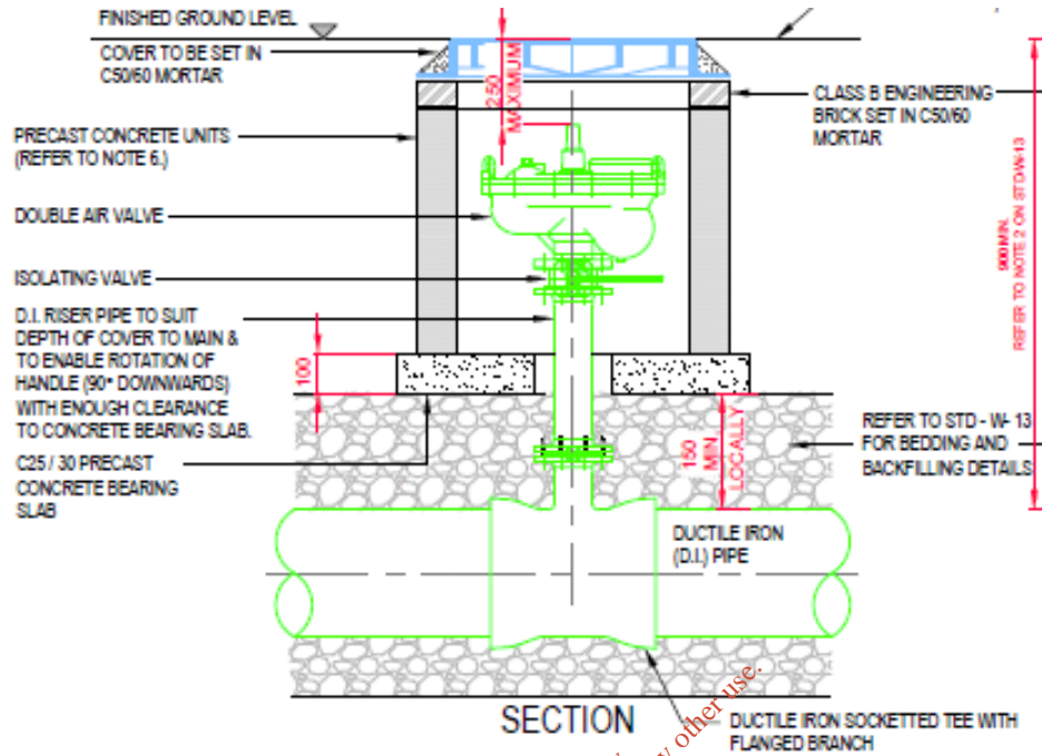
Typical Air Valve Arrangement
