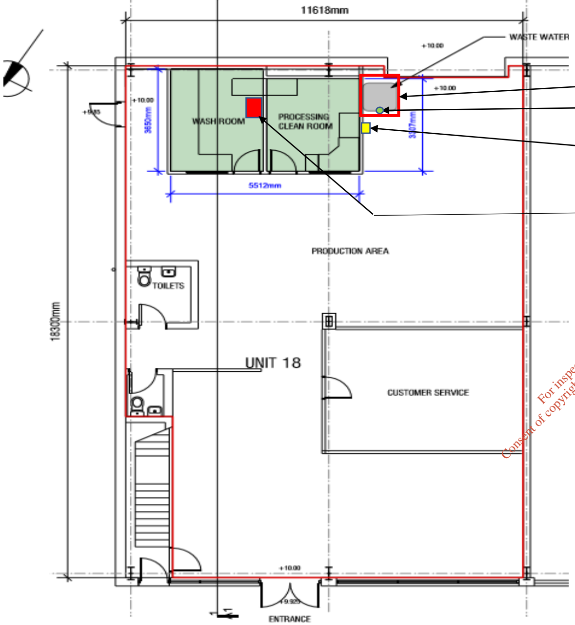
6 PROPOSED GROUND FLOOR PLAN Scale: 1:100
