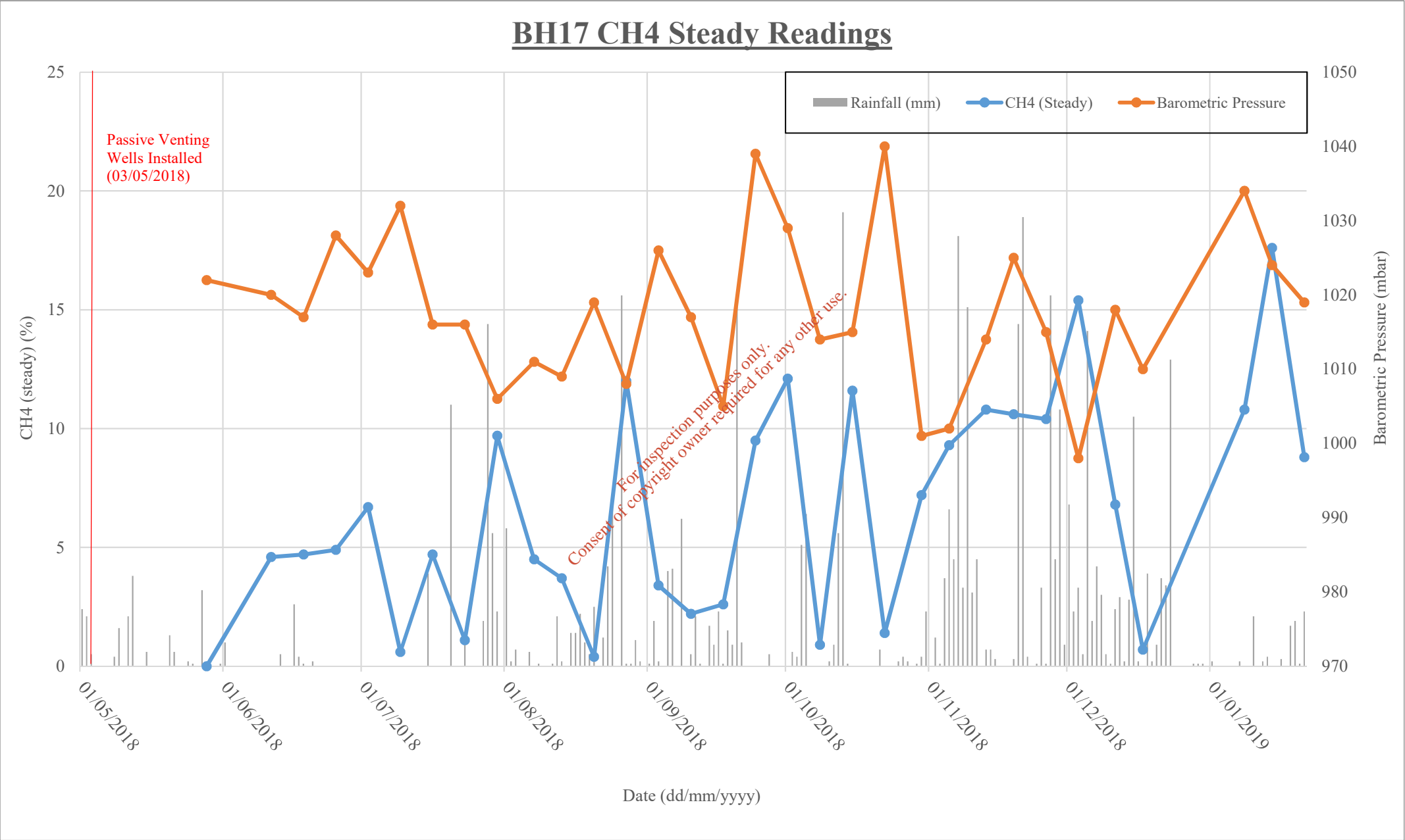
Chart 17. Methane (%) and Atmospheric Pressure (mbar) in Borehole BH17 (27/06/2017 - 26/06/2018)
