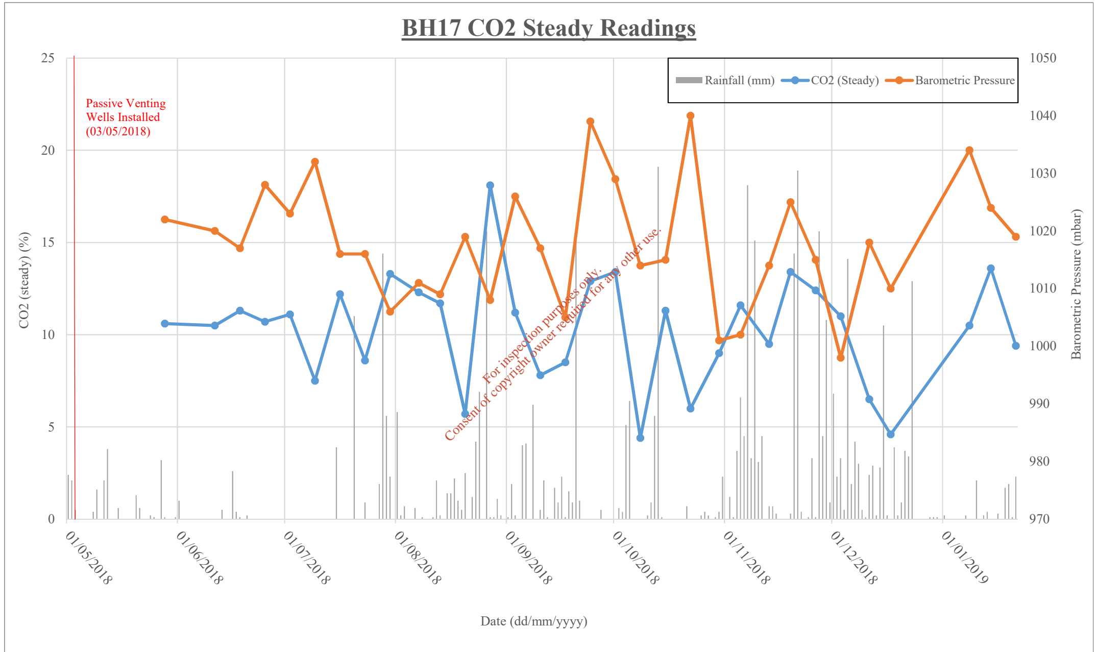
Chart 18. Carbon Dioxide (%) and Atmospheric Pressure (mbar) in Borehole 17 (27/06/2017 - 26/06/2018)
