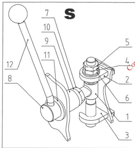
OPENING UNIT
