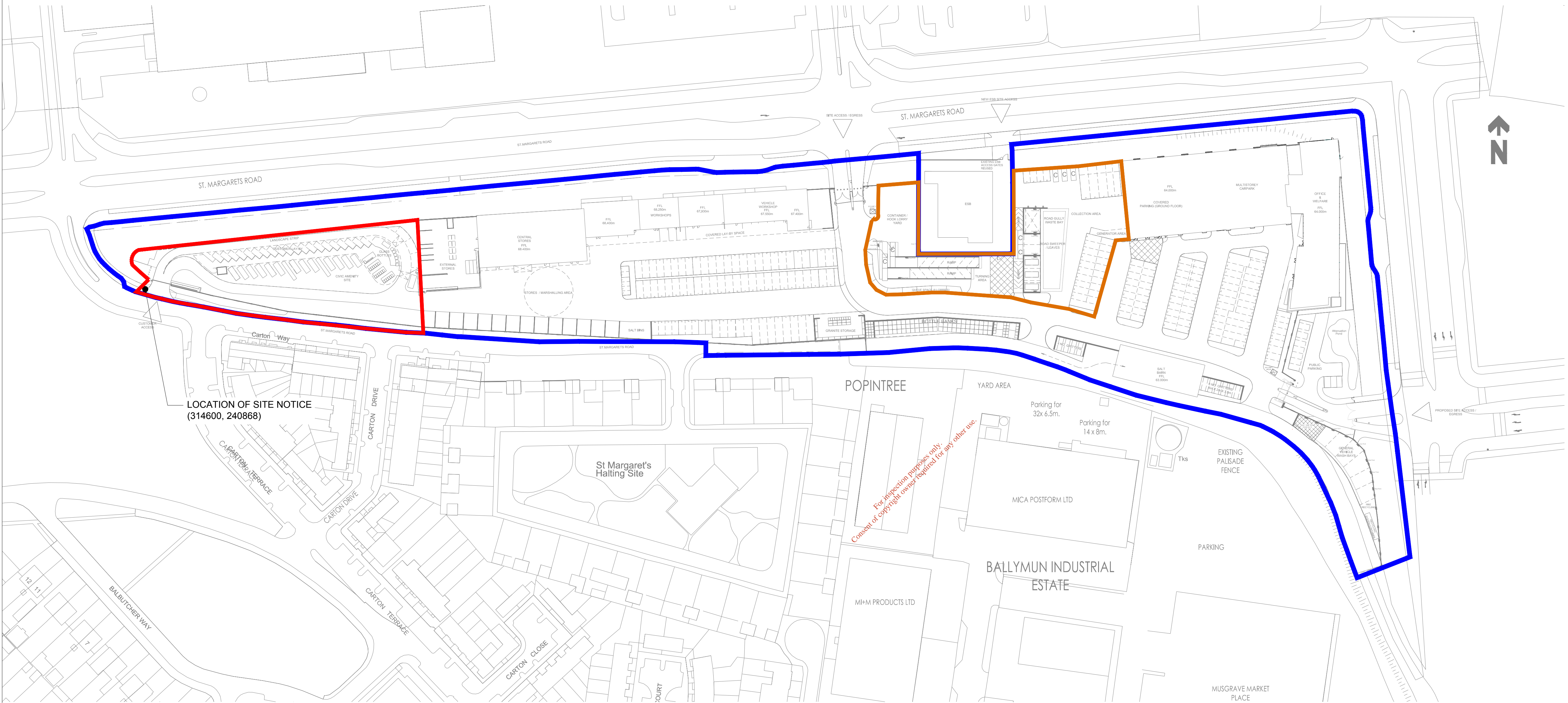
Waste Licence Site Notice Plan (Scale 1:1000)
