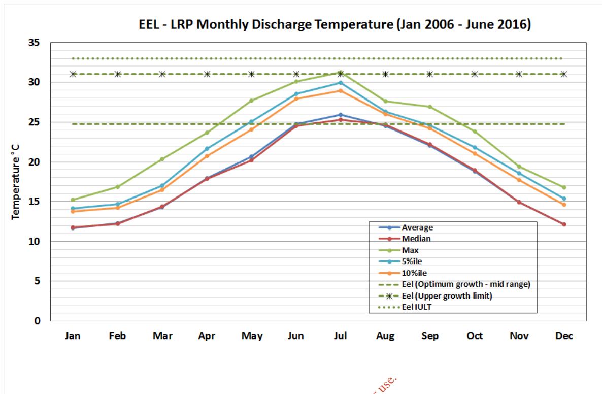
Figure 7b Eel thermal limits plotted against summarised seasonal discharge temperatures (2006-2016) at LRP
