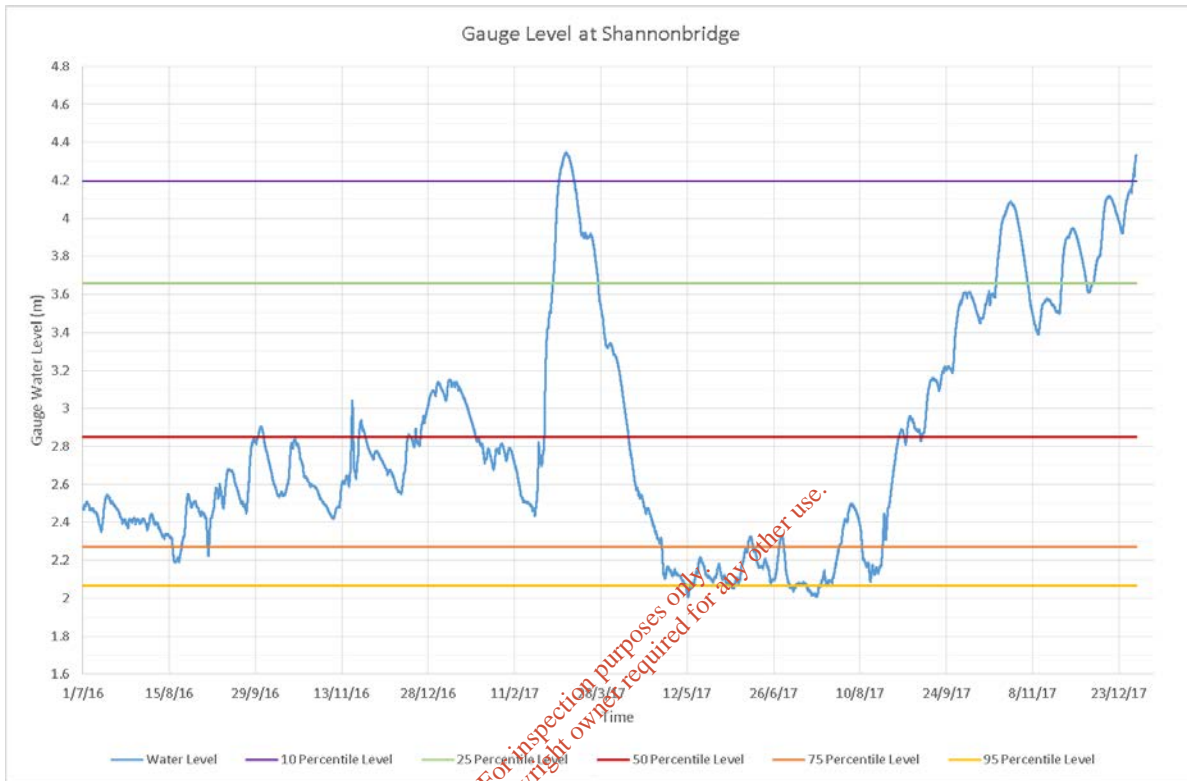
Figure 4-2 Water Levels at Shannonbridge (www.waterlevel.ie.)
