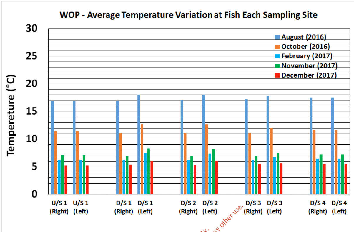
Figure 5-2 Average depth-averaged temperature at or nearby the 5 paired fyke net sampling stations at WOP for each of the 5 fishing surveys. (Data extracted from IHD temperature monitoring reports).
