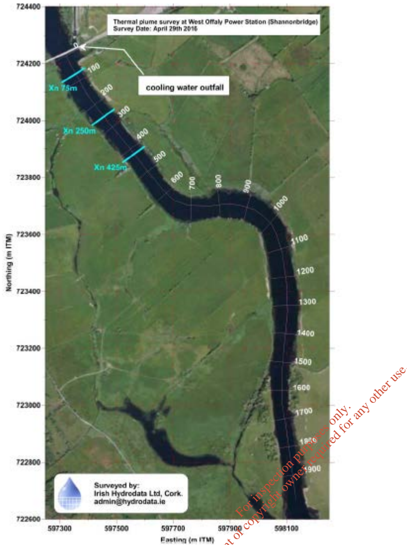
Figure 2-3 Location of River Shannon cross-sections at Shannonbridge (IHD)
