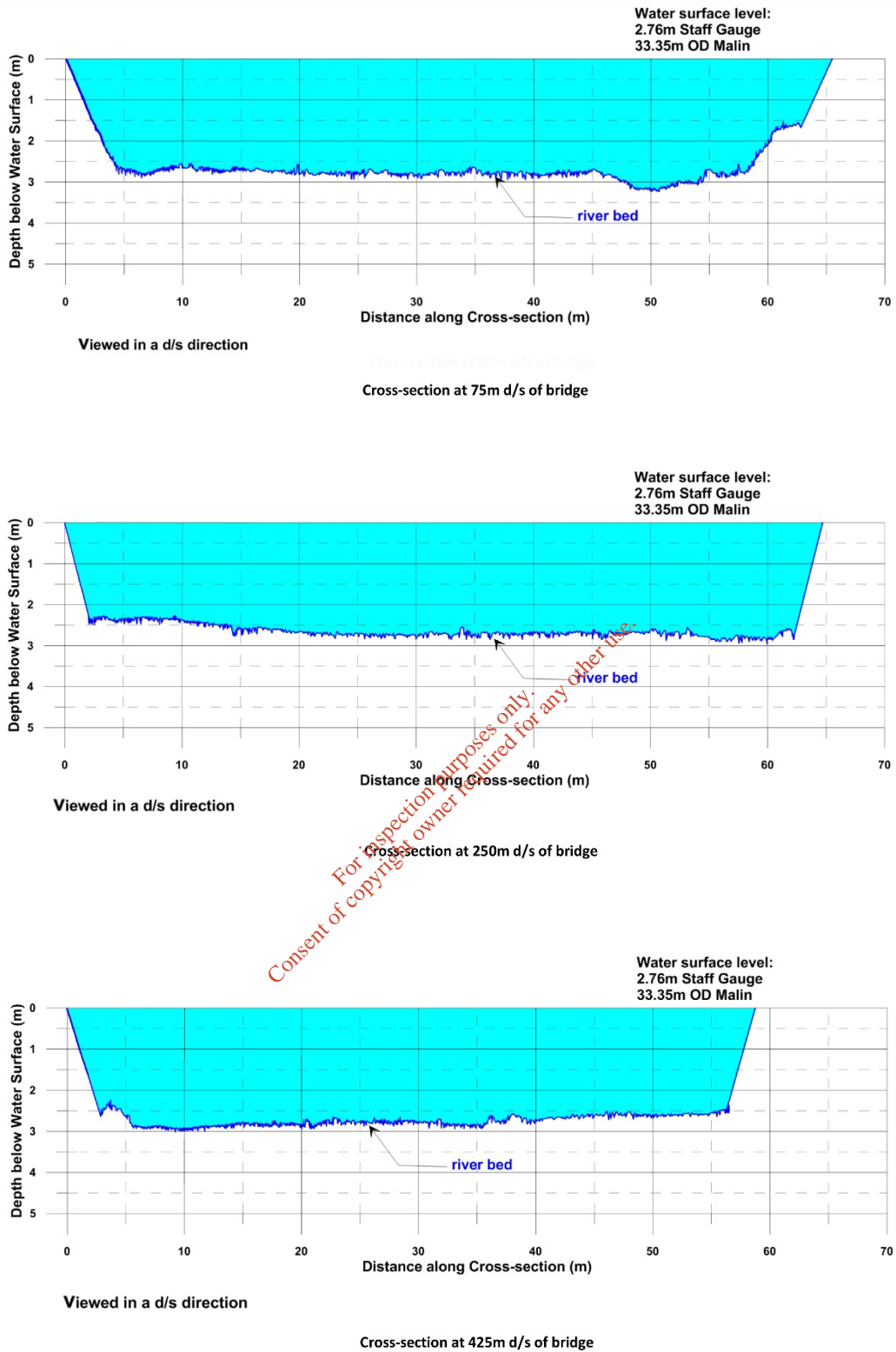
Figure 2-2 River Shannon cross-sections at Shannonbridge
