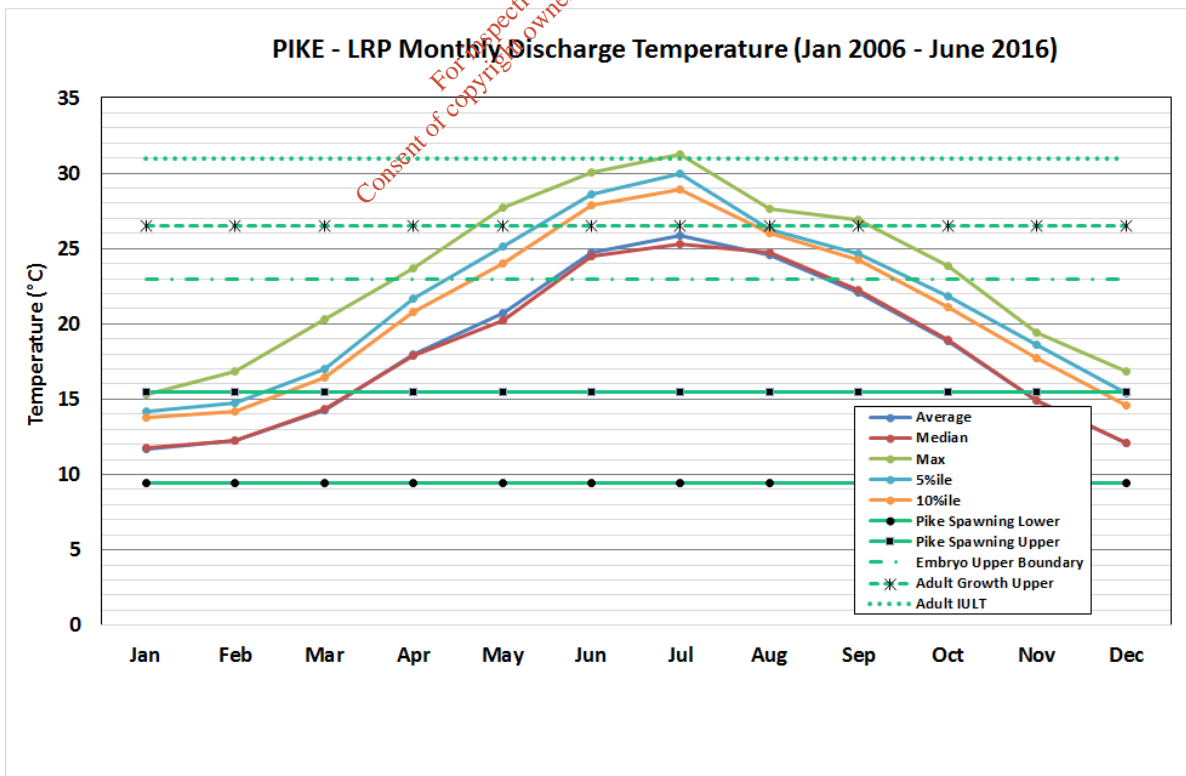
Figure 11b Pike thermal limits plotted against summarised seasonal discharge temperatures (2006-2016) at LRP
