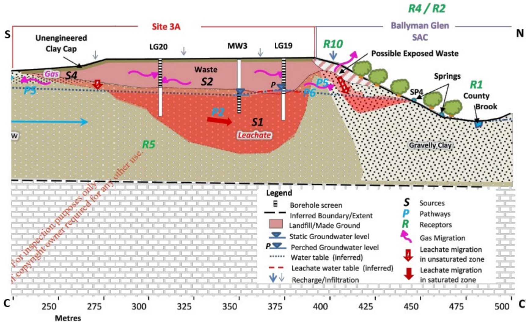
Figure 4 Conceptual site model for Fassaroe 3A site
