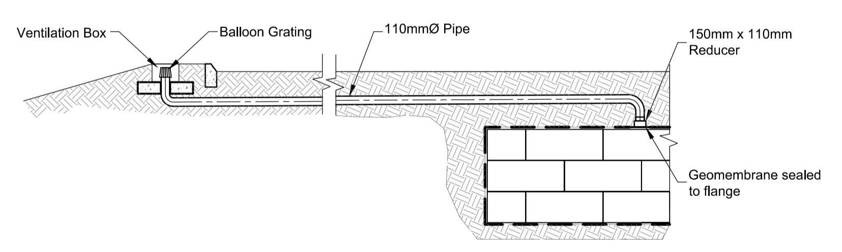
Typical Section Through Air Vent Scale: 1:50
