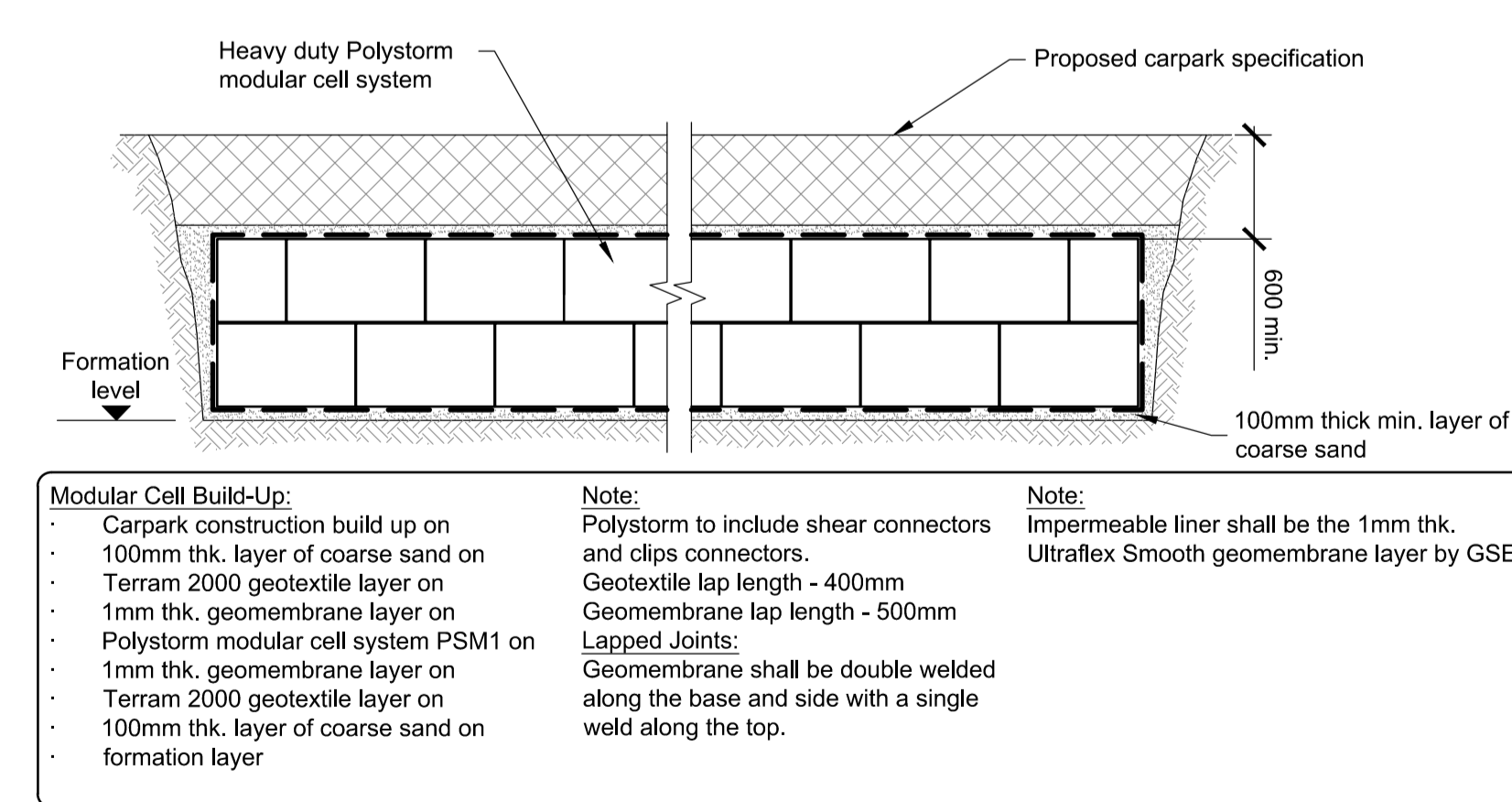
Proposed Polypipe Polystorm Modular Cell System Scale: 1:50
