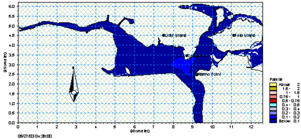
Figure A 5.19 Phosphate, high tide, Sim. No 2 –no Carrigtohill input (Plot units mg/l)
