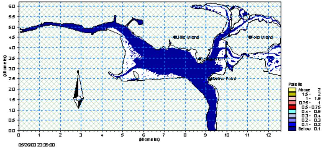
Figure A 5.22 Phosphate, low tide, Sim. No 2 –no Carrigtohill input (Plot units mg/l)
