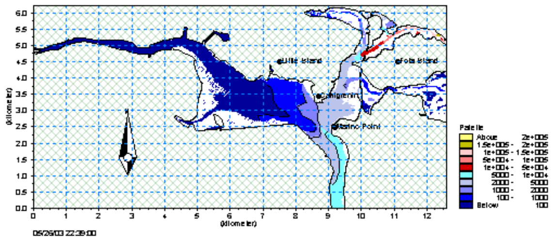
Figure A5.6 Total Coliforms, low tide, Sim. No 9 –combined input (Plot units /100ml)
