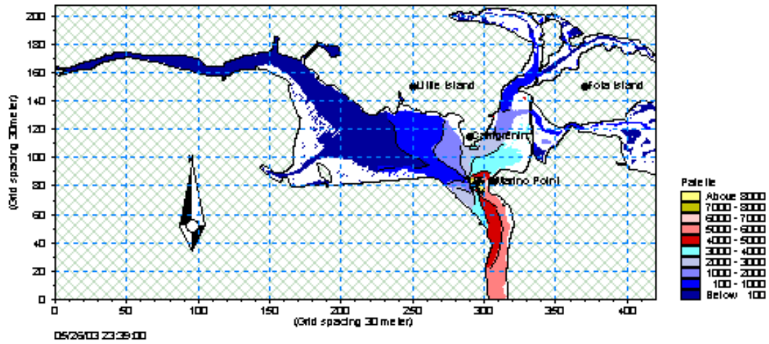
Figure A 5.4 Total Coliforms, low tide, Sim. No 2 –no Carrigtohill input (Plot units / 100ml)
