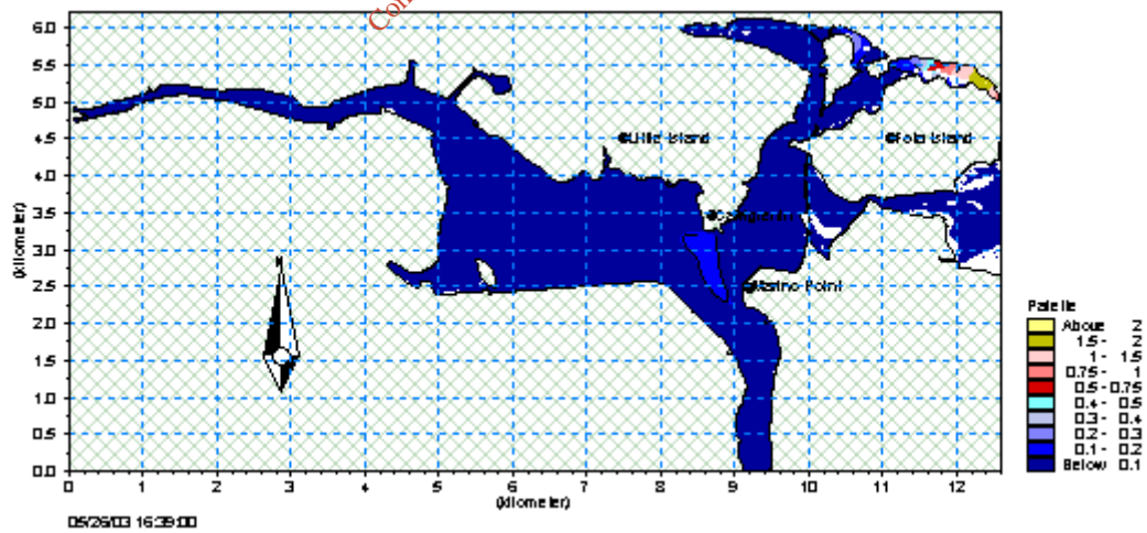
Figure A 5.21 Phosphate, high tide, Sim. No 9 –combined input (Plot units mg/l)
