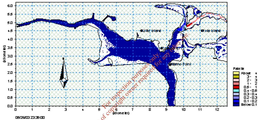
Figure 5.11 BOD, low tide, Sim. No 4 –no Carrigrenan input (Plot units mg/l)
