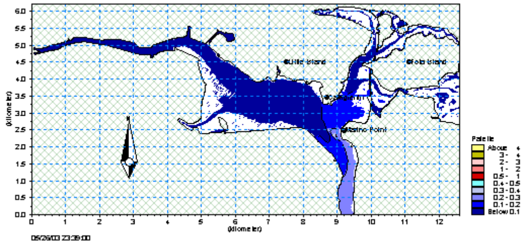
Figure A2.10 BOD, low tide, Sim. No 2 –no Carrigtohill input (Plot units mg/l)
