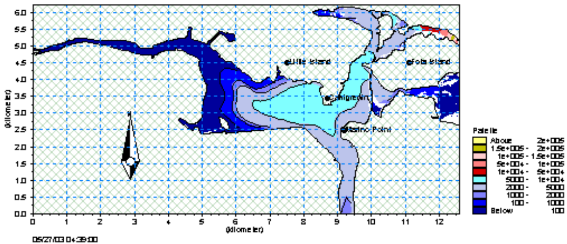
Figure A 5.3 Total Coliforms, high tide, Sim. No 9 –combined input Plot units / 100ml)
