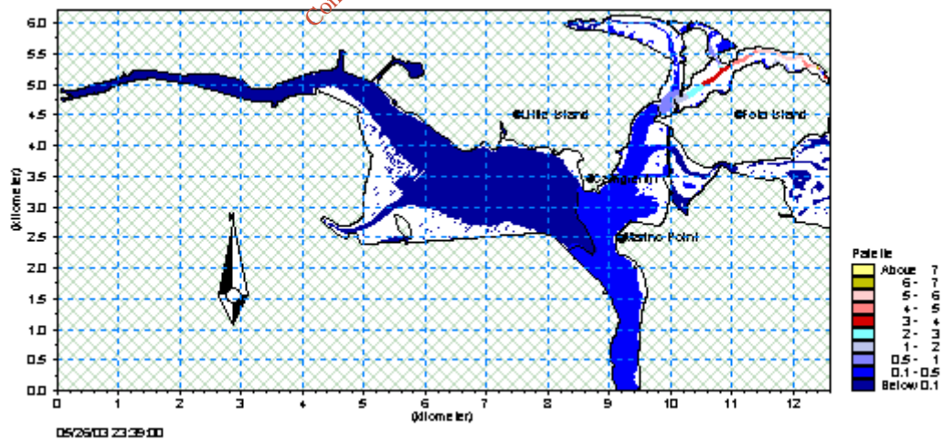
Figure A 5.18 Nitrate, low tide, Sim. No 9 –combined input (Plot units mg/l)
