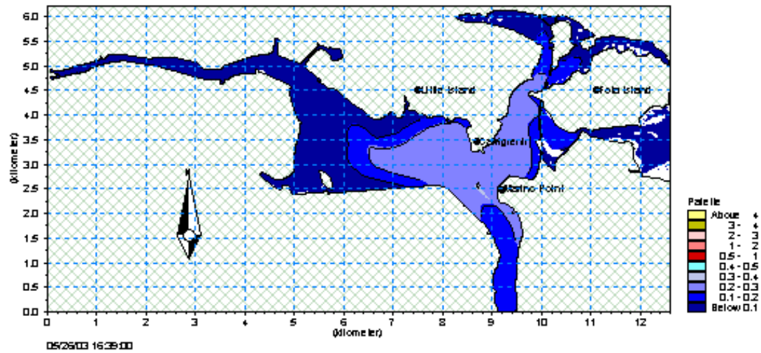
Figure A5.7 BOD, high tide, Sim. No 2 –no Carrigtohill input (Plot units mg/l)
