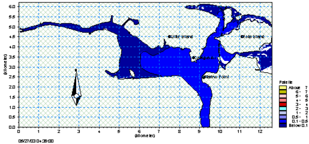
Figure A5.13 Nitrate, high tide, Sim. No 2 –no Carrigtohill input (Plot units mg/l)
