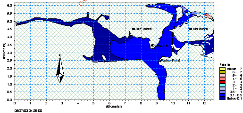
Figure 5.15 Nitrate, high tide, Sim. No 9 –combined input (Plot units mg/l)
