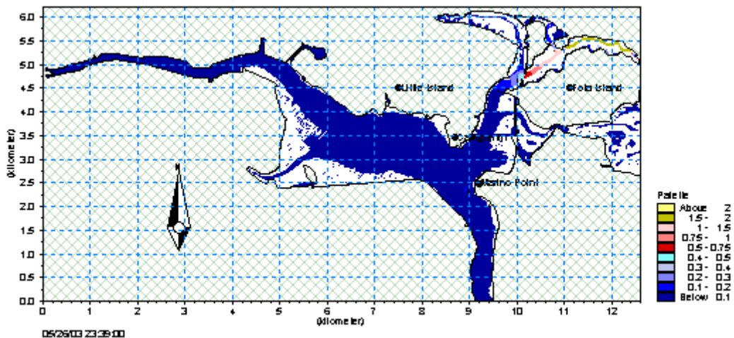
Figure A 5.24 Phosphate, low tide, Sim. No 9 –combined input (Plot units mg/l)
