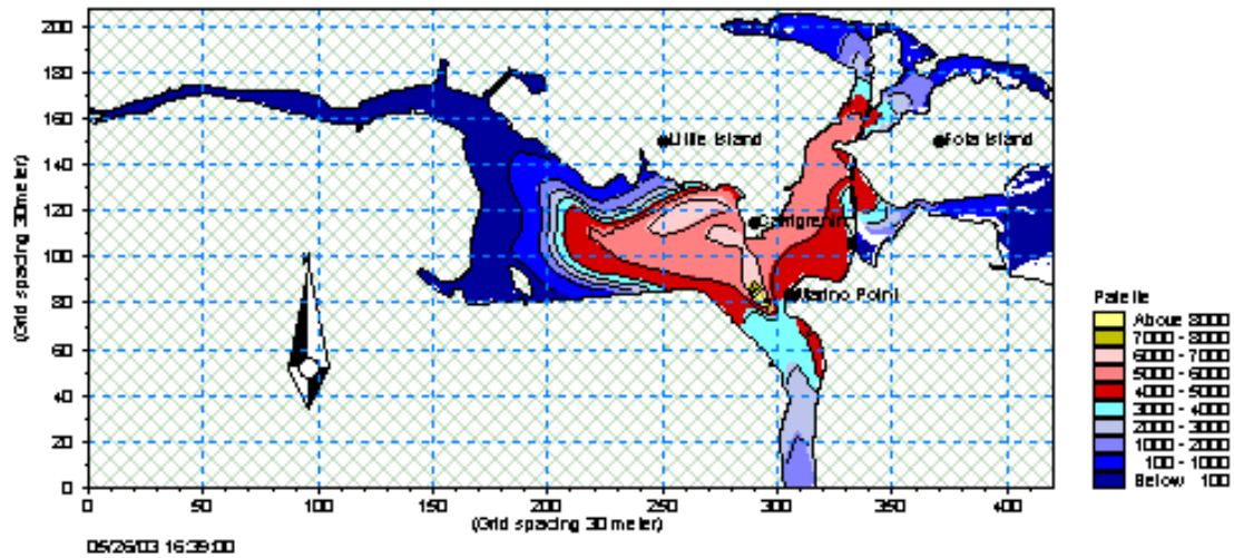
Figure A 5.1 Total Coliforms, high tide, Sim. No 2 –no Carrigtohill input (Plot Units / 100mls)
