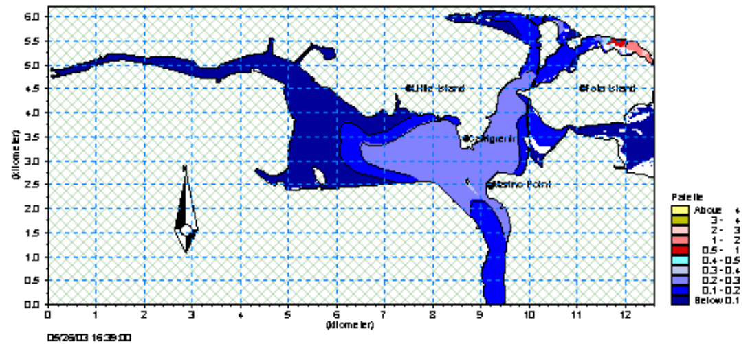
Figure A5.9 BOD, high tide, Sim. No 9 –combined input (Plot units mg/l)
