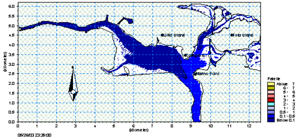
Figure A 5.16 Nitrate, low tide, Sim. No 2 –no Carrigtohill input (Plot units mg/l)
