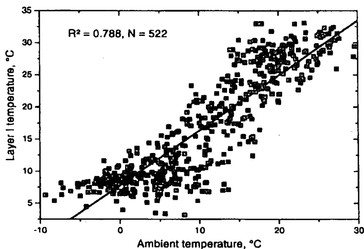
Fig. 7. Recorded ambient temperature plotted vs. recorded temperature in layer I (shown is the regression line).
