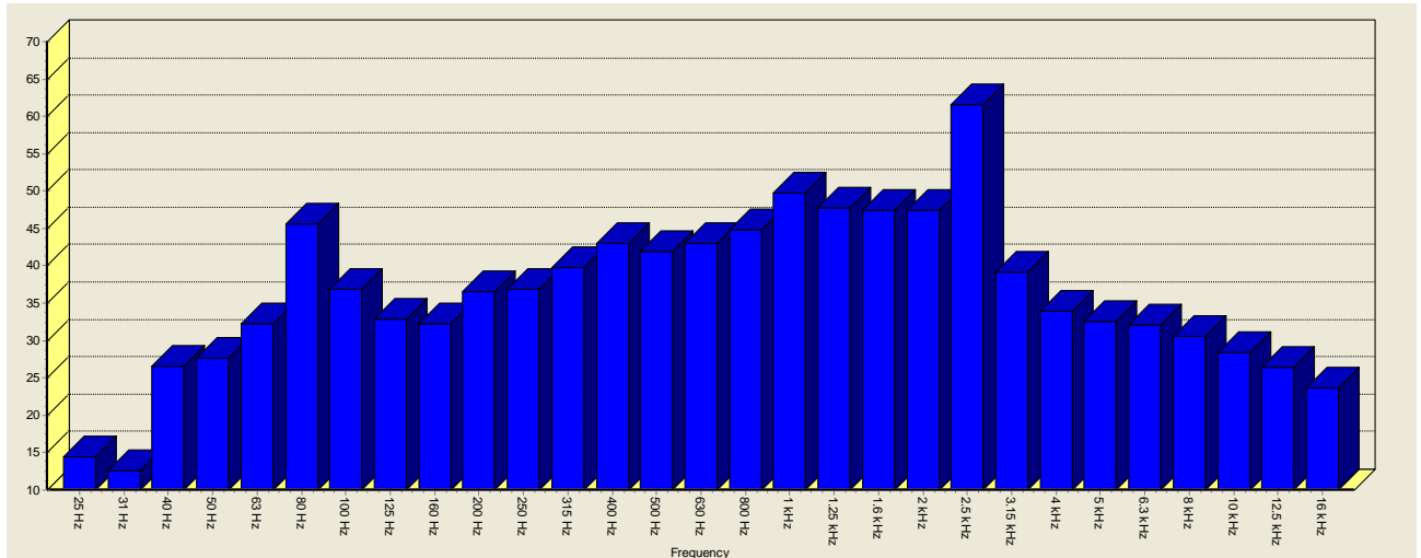
Fig 1. Location N1. 1/3 octave analysis A weighted
