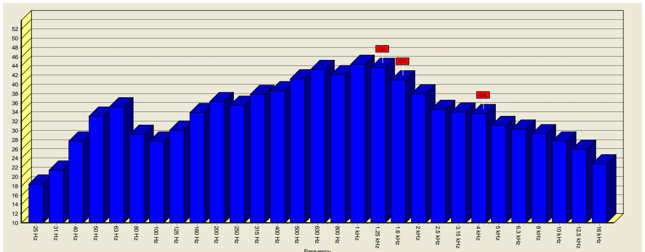
Fig 2. Location N4. 1/3 octave analysis A weighted.
