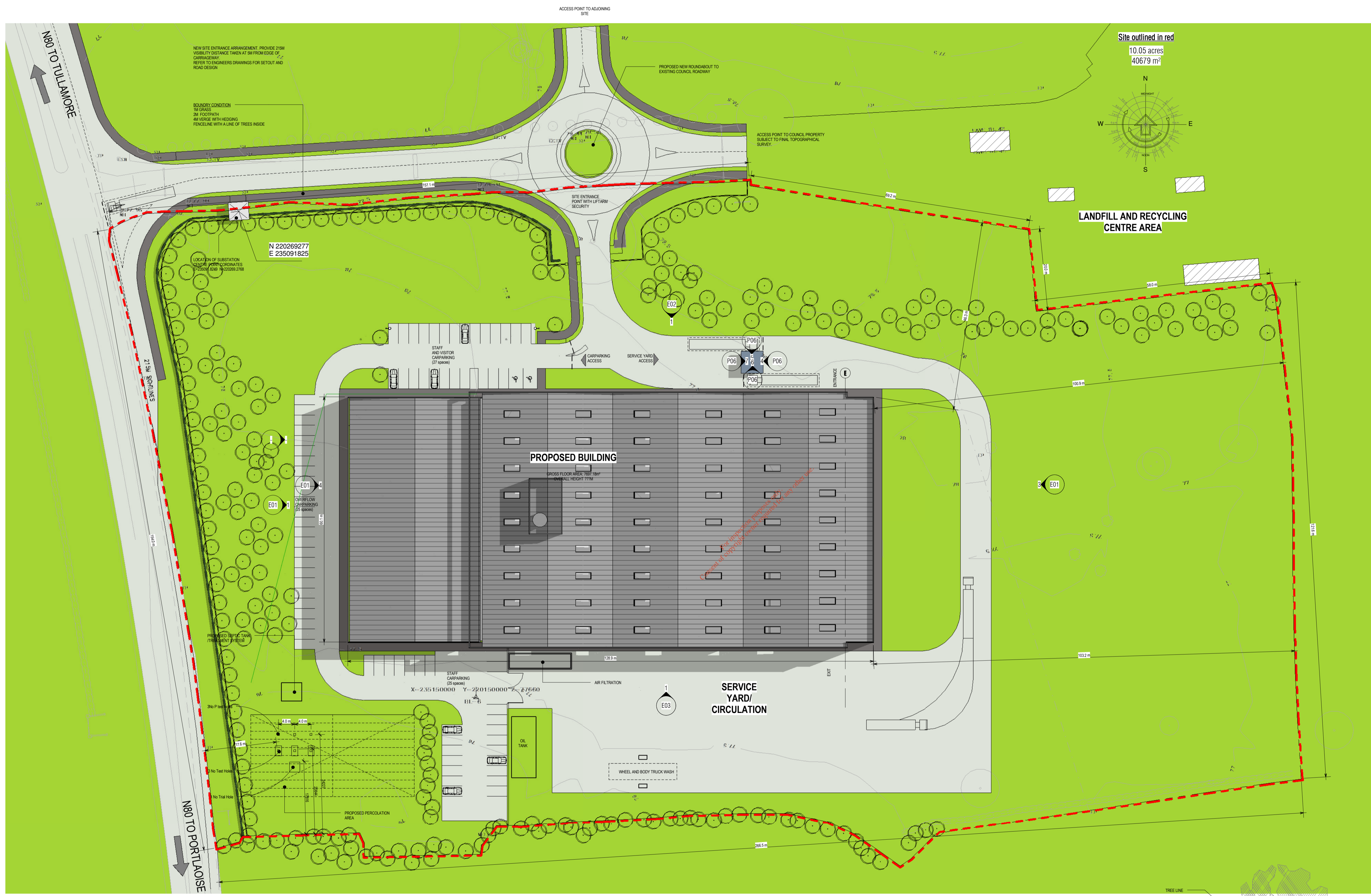
1 Site layout Plan 1:500 RE: 1/E01
