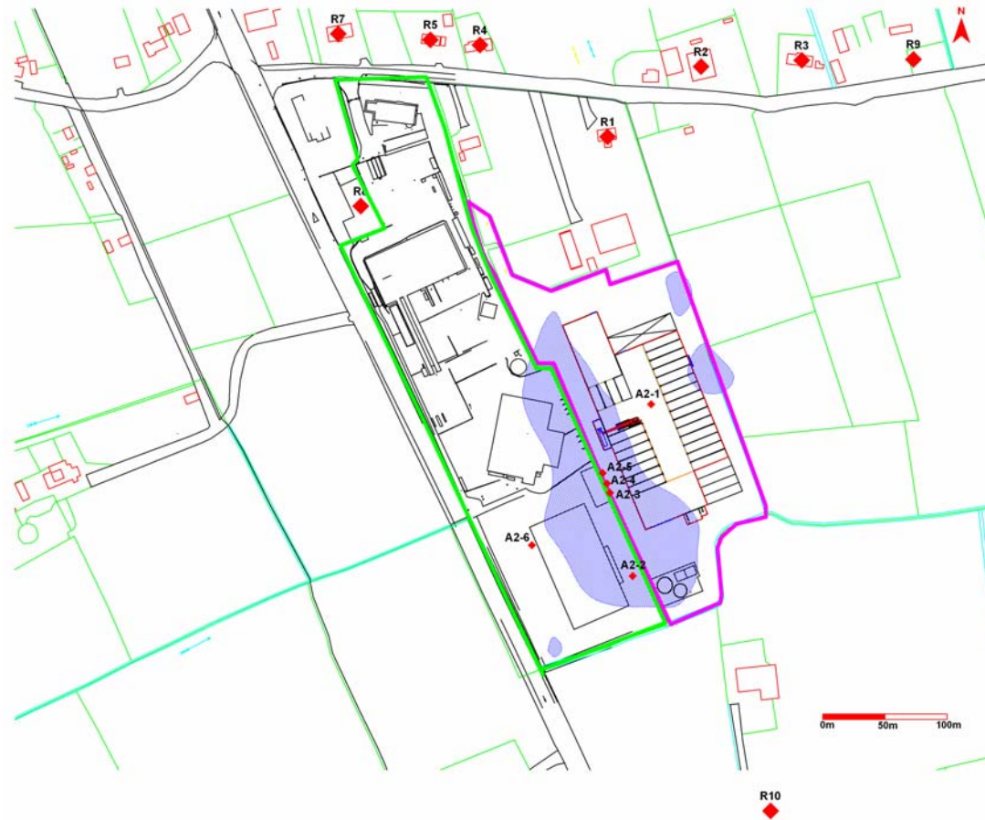
Figure 8.2. Predicted odour emission contribution of proposed overall Panda Waste Dry Fermentation and RDF Facility operation to odour plume dispersal for the 98 th percentile for an odour concentration of \leq 1.50 \text{ Ou}_E \text{ m}^{-3} ( — ) for worst case meteorological year Dublin 2004.
