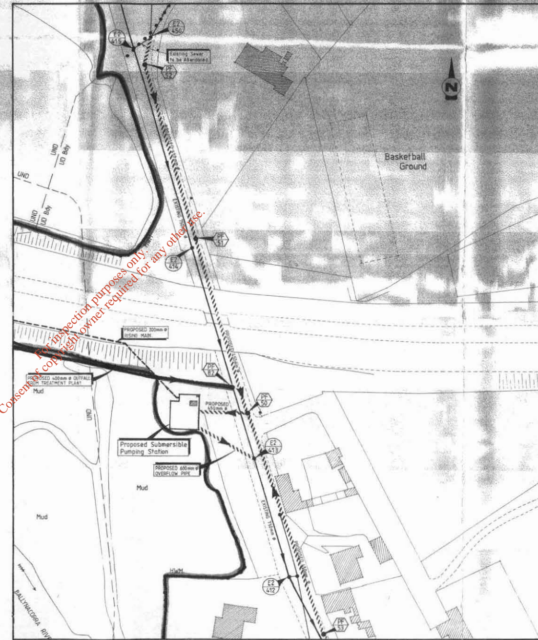
1:500 LAYOUT PLAN
