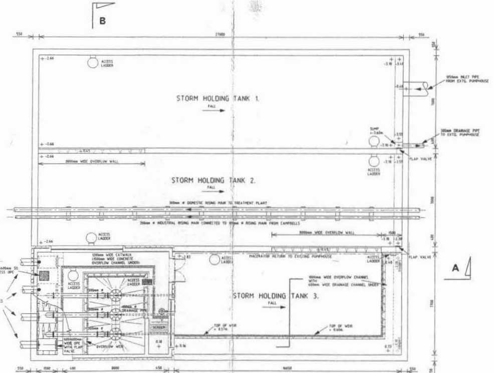
SECTIONAL PLAN
