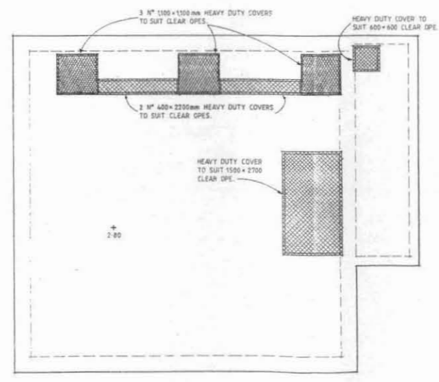
ROOF PLAN 1/50
