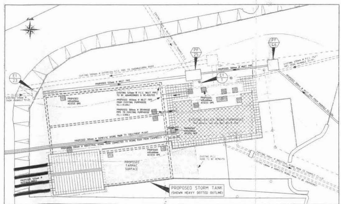
1/200 LAYOUT PLAN
