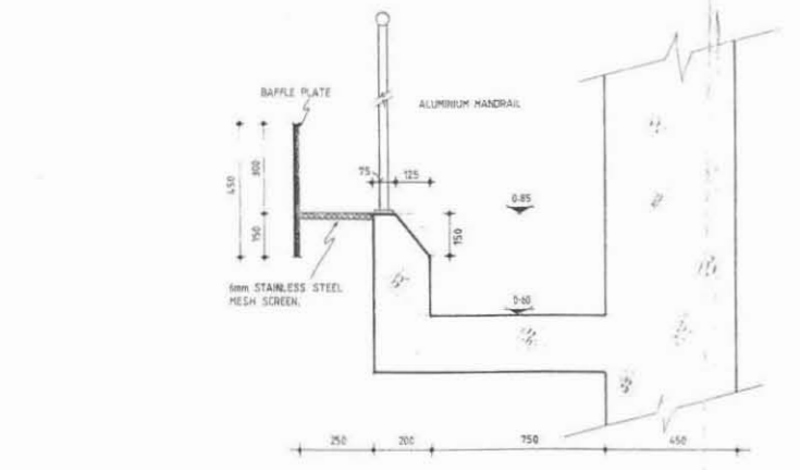
SECTION B-B 1/50
