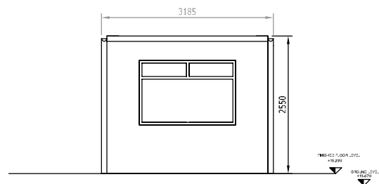
SOUTHWEST ELEVATION
