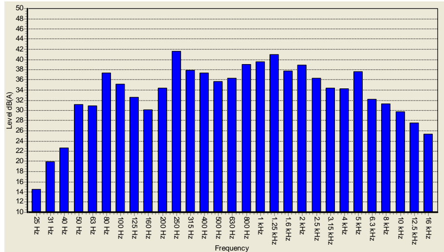
Fig 1. Location N1. 1/3 octave analysis A weighted.
