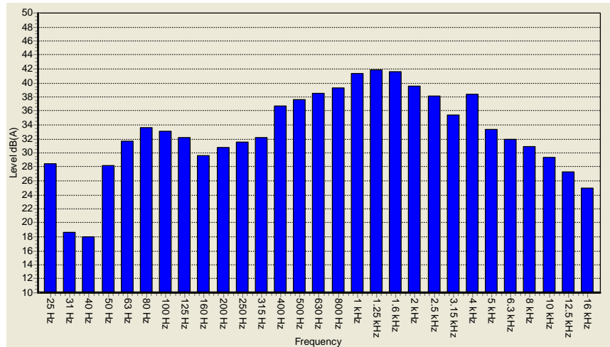
Fig 4. Location N4 1/3 octave analysis A weighted.
