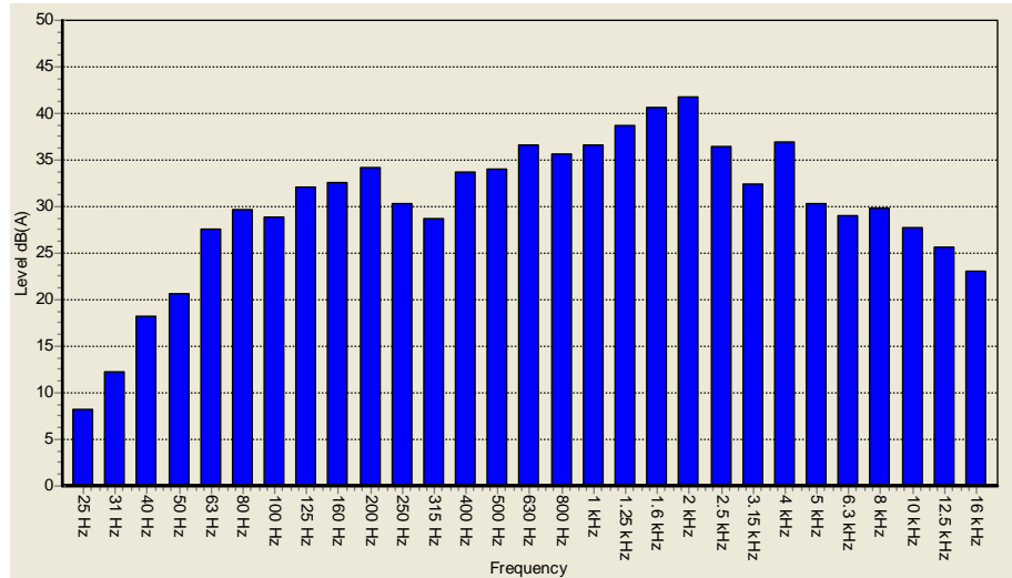
Fig 2. Location N2. 1/3 octave analysis A weighted.
