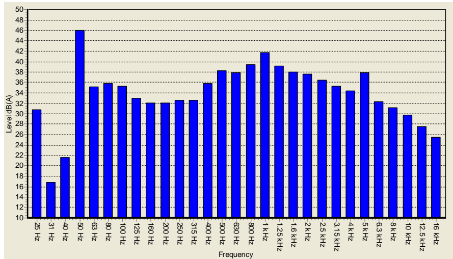
Fig 3. Location N3 1/3 octave analysis A weighted.
