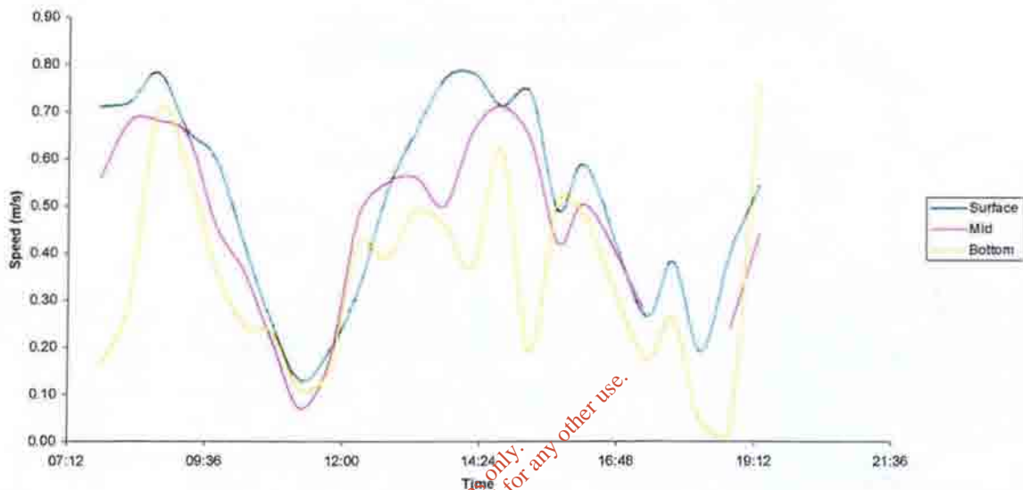
Site A Neap Tide Current Speeds 13/06/01
