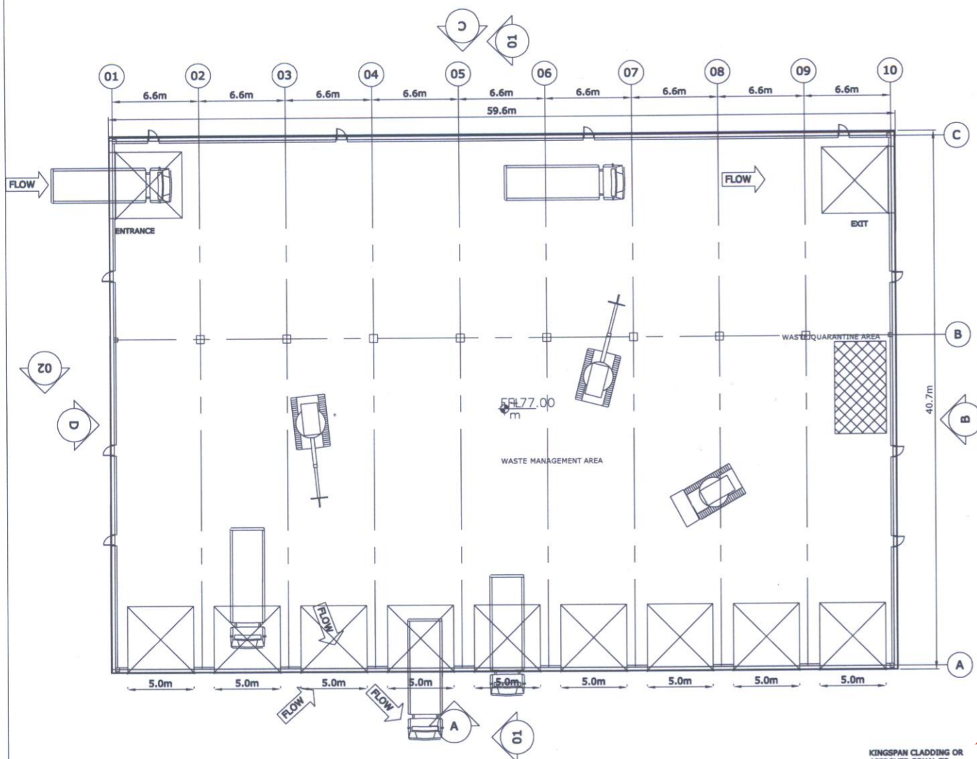
PLAN ON WASTE TRANSFER FACILITY
