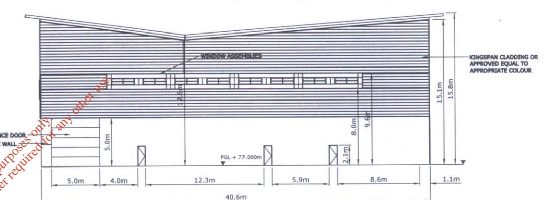
ELEVATION D
