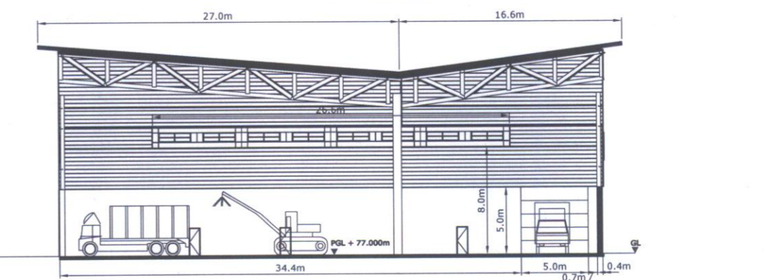
SECTION ON 01
