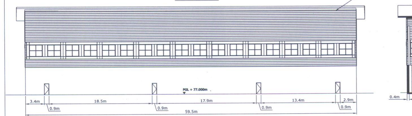
ELEVATION C
