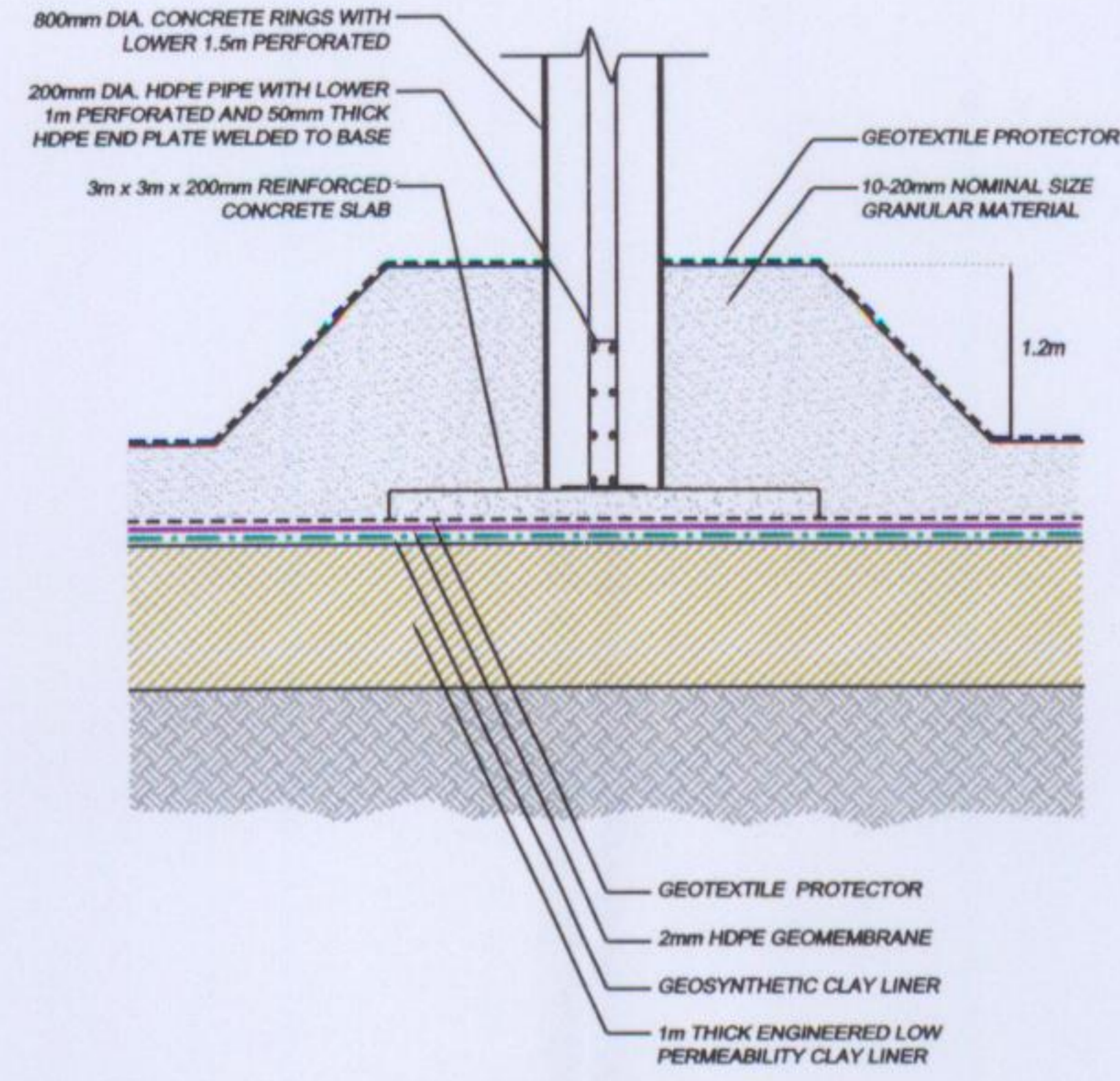
SECTION C-C THROUGH LEACHATE MONITORING WELL
