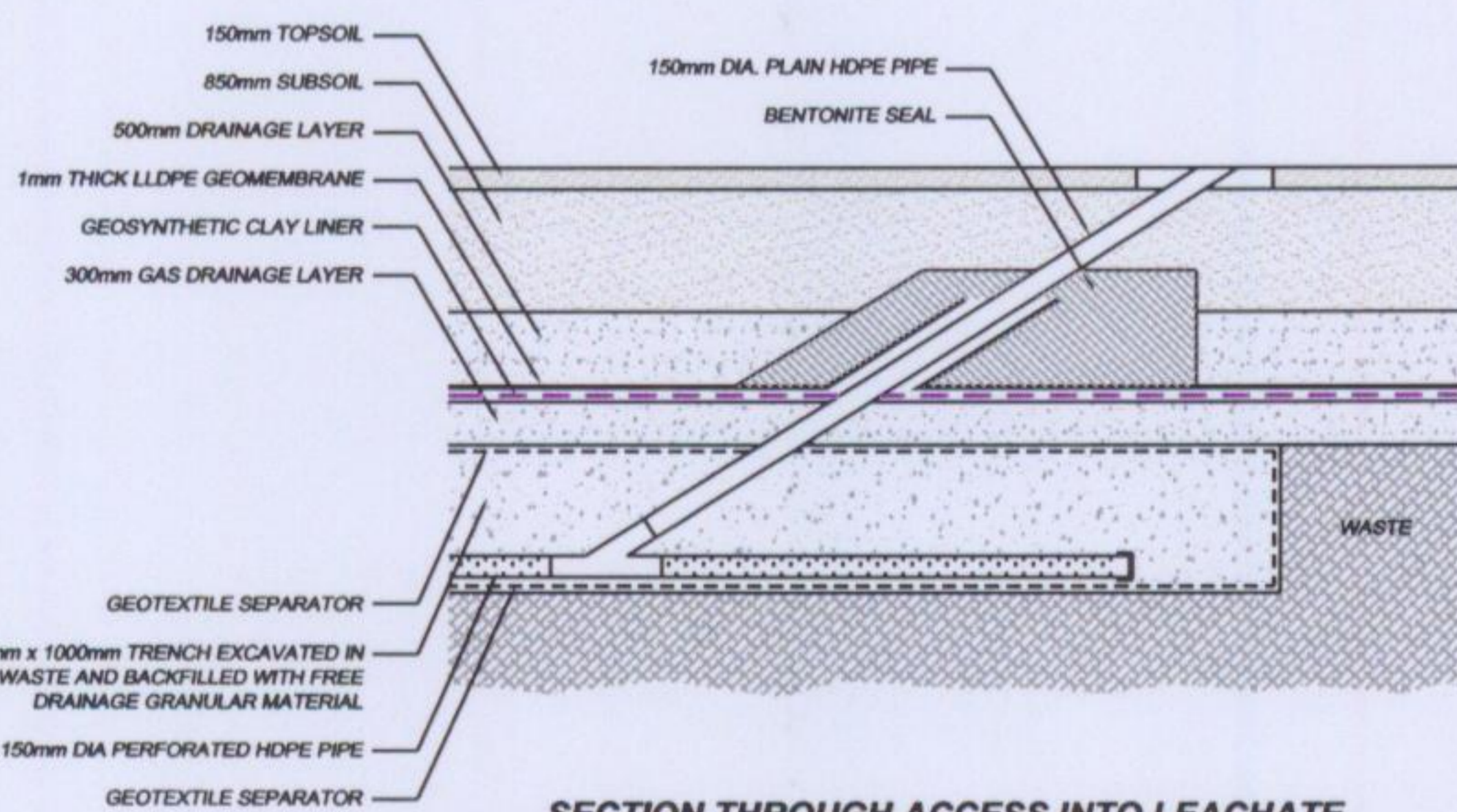
SECTION THROUGH ACCESS INTO LEACHATE RECIRCULATION SYSTEM (GEOSYNTHETIC CAP OPTION) 1:100
