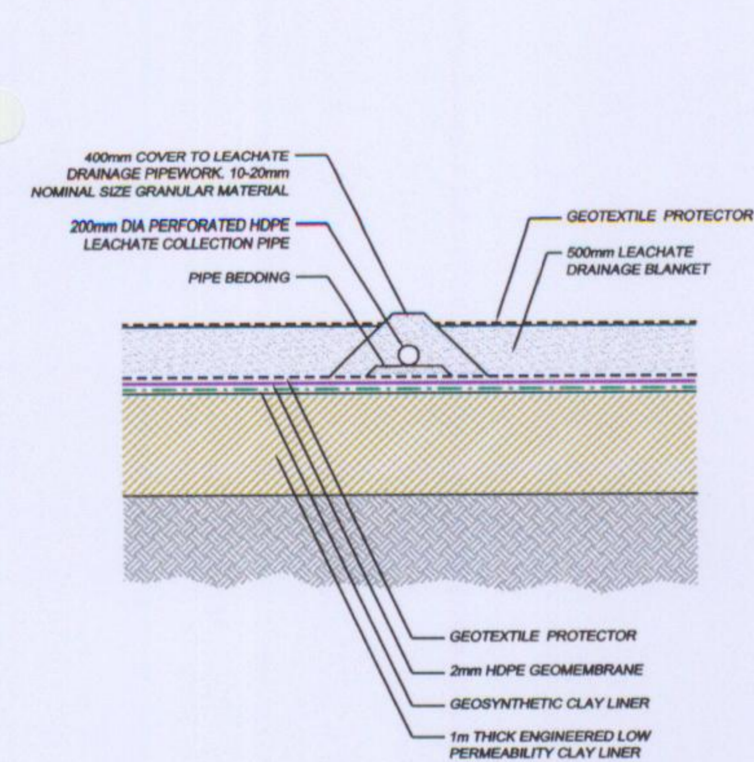
SECTION A-A THROUGH LEACHATE COLLECTION PIPEWORK
