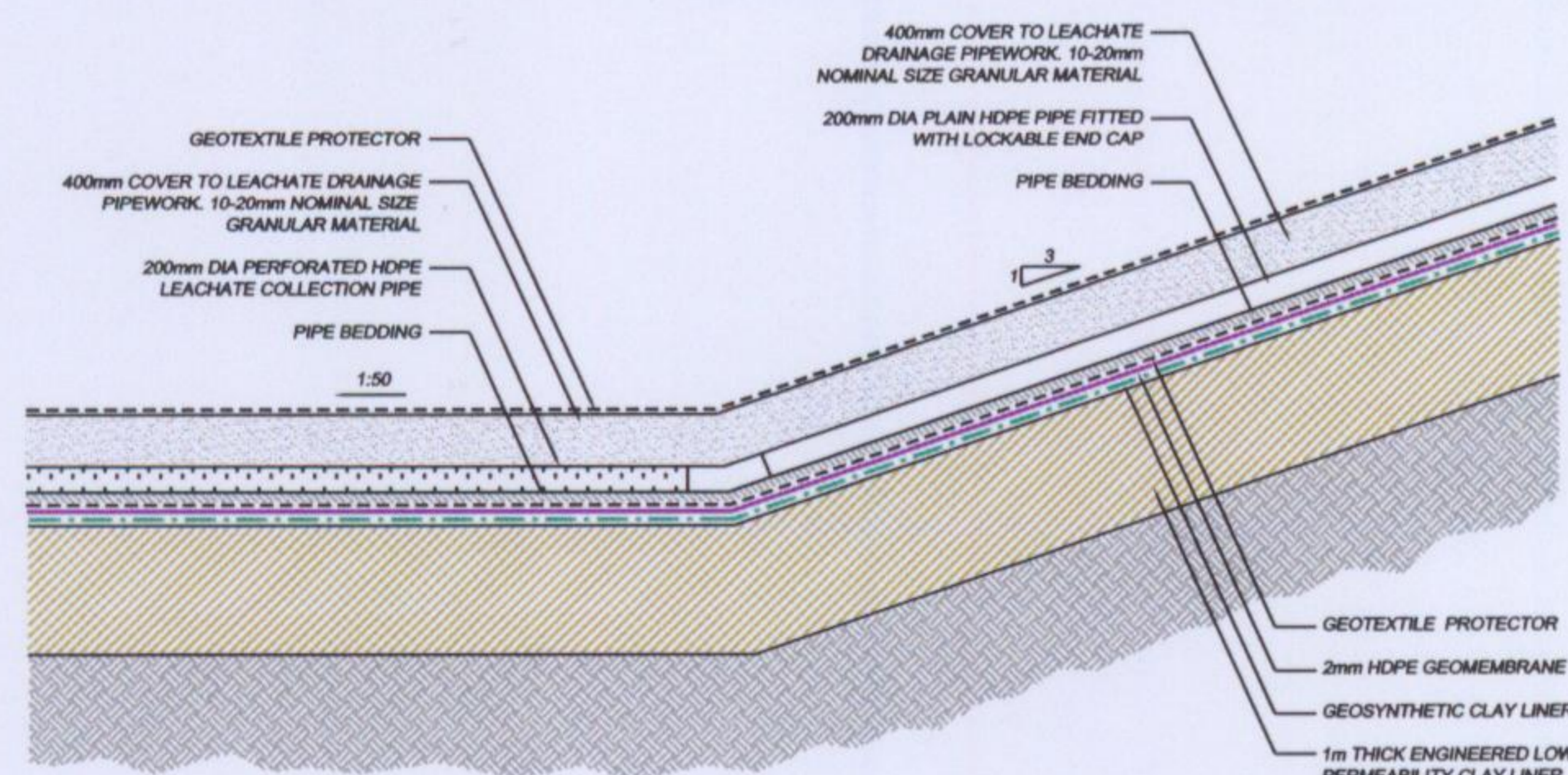
SECTION E-E THROUGH LEACHATE COLLECTION DRAIN AT BASE OF SIDESLOPE
