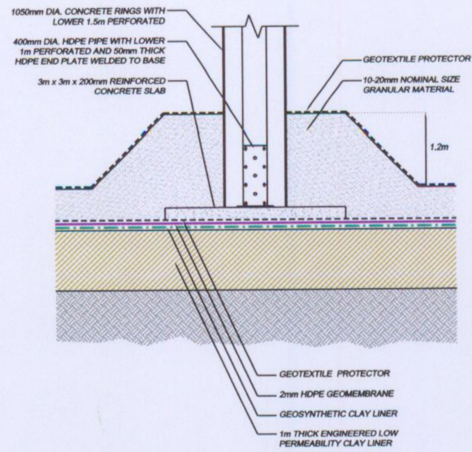
SECTION B-B THROUGH LEACHATE EXTRACTION WELL
