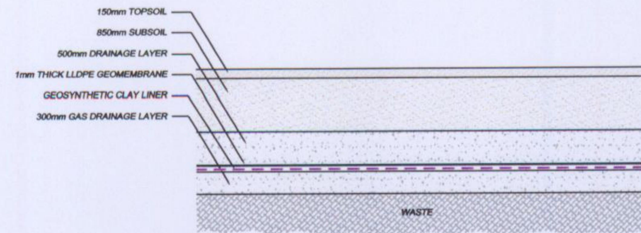
SECTION THROUGH GEOSYNTHETIC CAPPING SYSTEM 1:100
