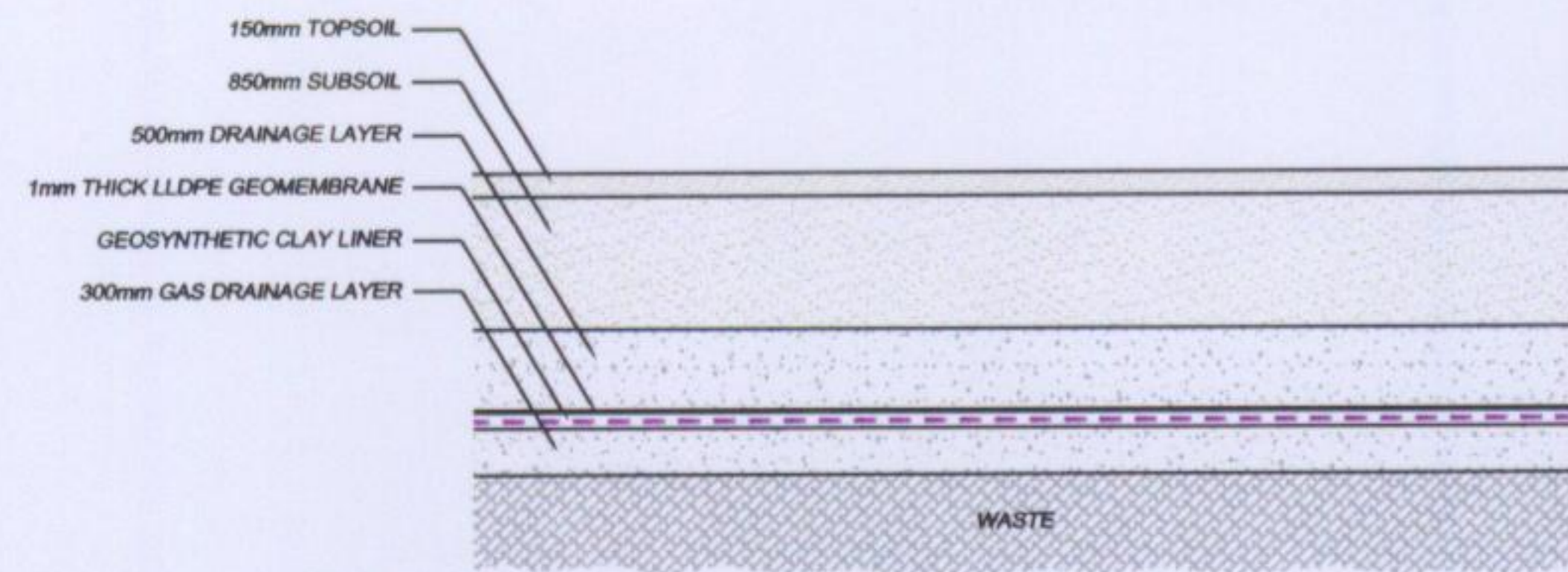
SECTION THROUGH CAPPING SYSTEM T:100
