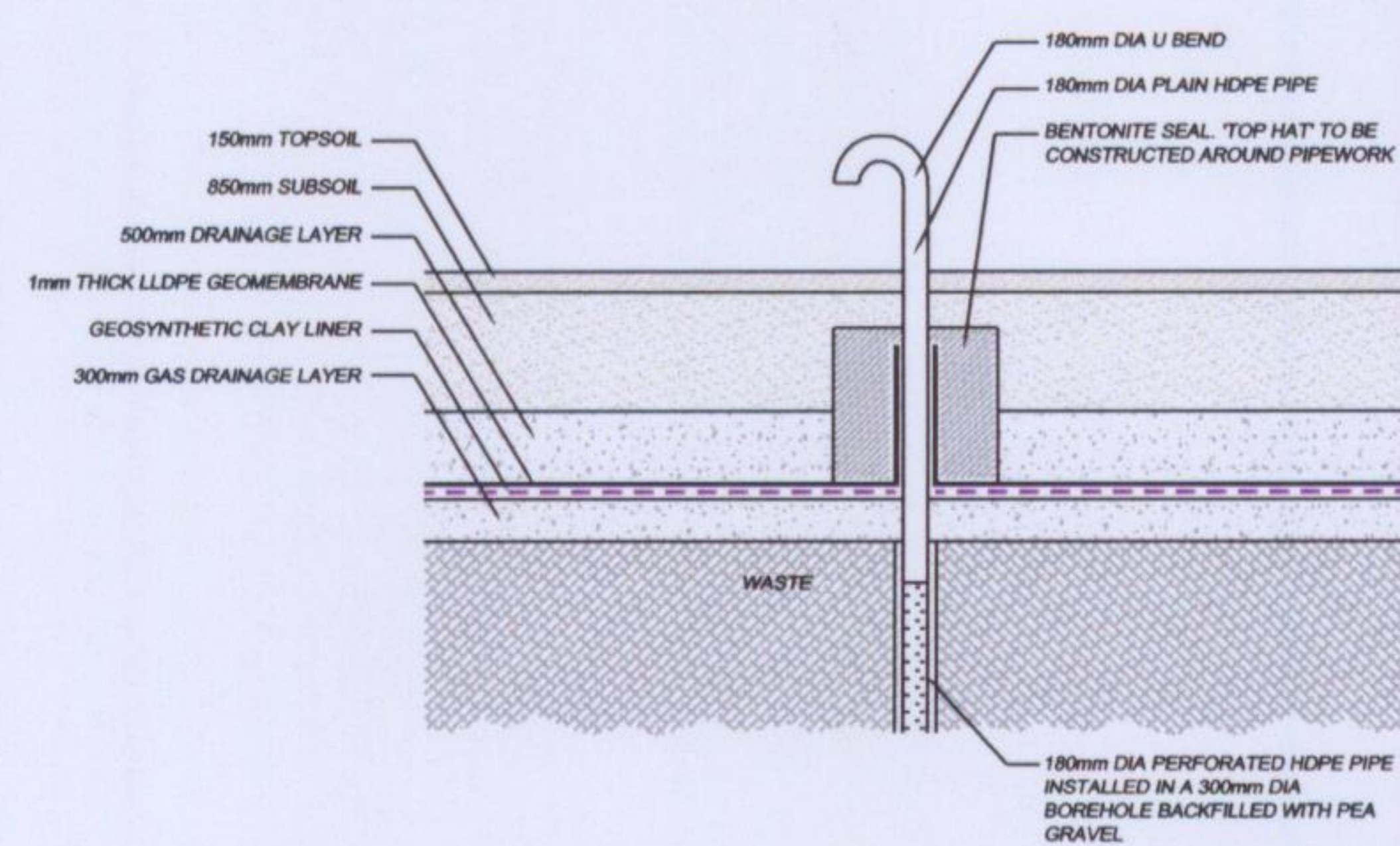
SECTION THROUGH DEEP GAS WELL PROTRUSION THROUGH CAPPING SYSTEM T:100
