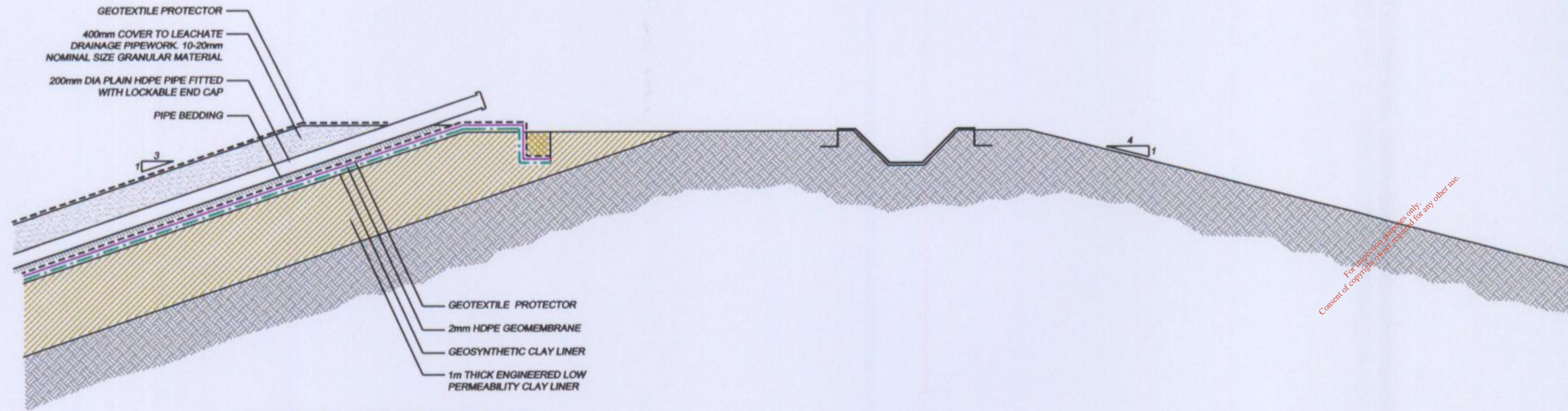
SECTION D-D THROUGH LEACHATE COLLECTION DRAIN AT CREST OF SIDESLOPE
