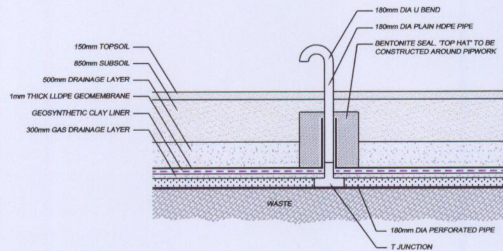
SECTION THROUGH GAS WELL CONNECTED INTO THE GAS DRAINAGE LAYER T:100
