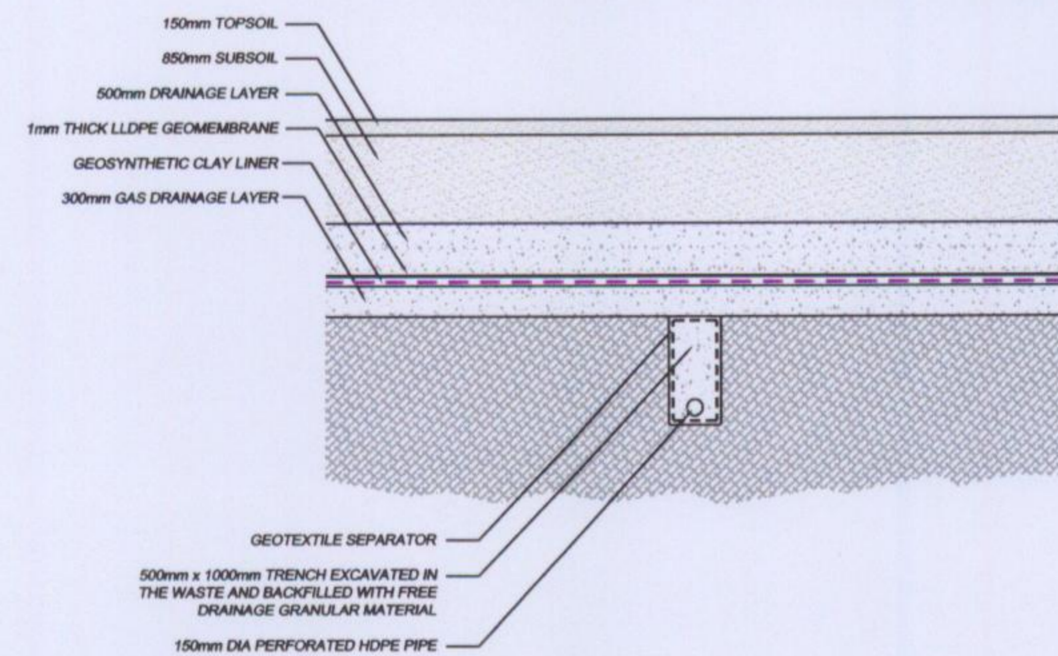
SECTION THROUGH LEACHATE RECIRCULATION TRENCH (GEOSYNTHETIC CAP OPTION) 1:100
