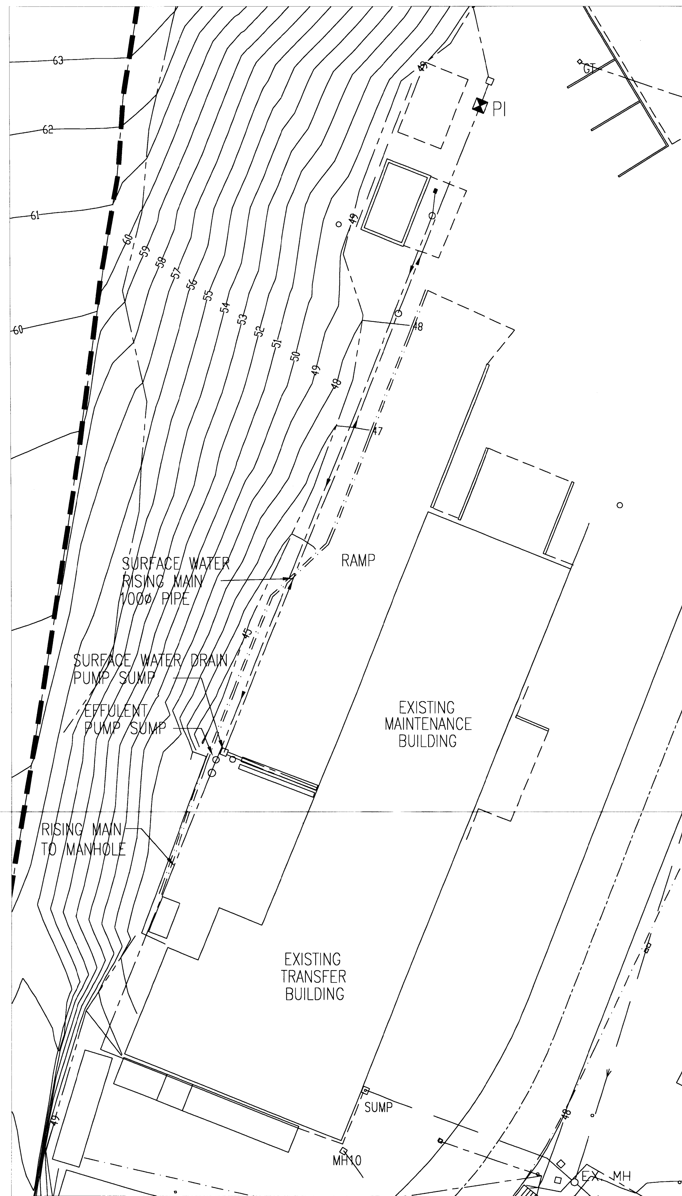
EXISTING DRAINAGE AT QUARANTINE AREA/TRUCK WASH AREA
