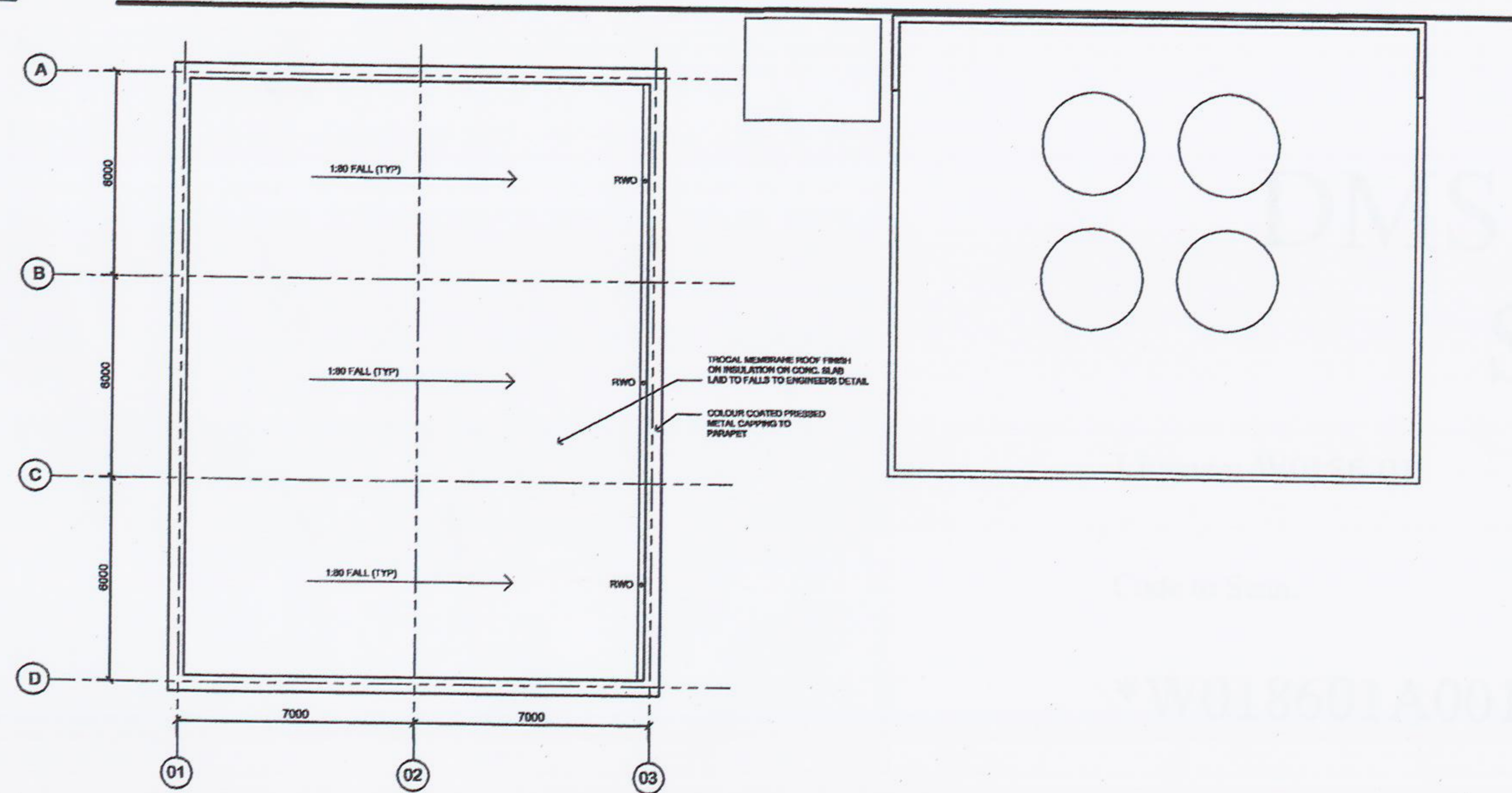
ROOF PLAN - DRUM WASH
