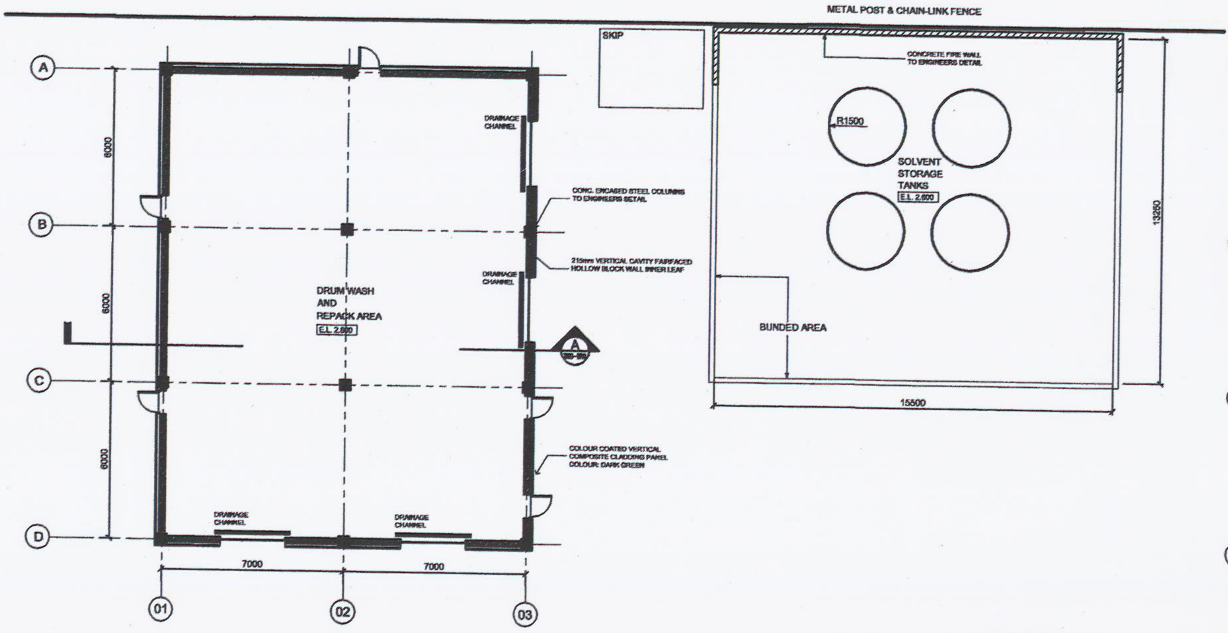
GROUND FLOOR PLAN - DRUM WASH
