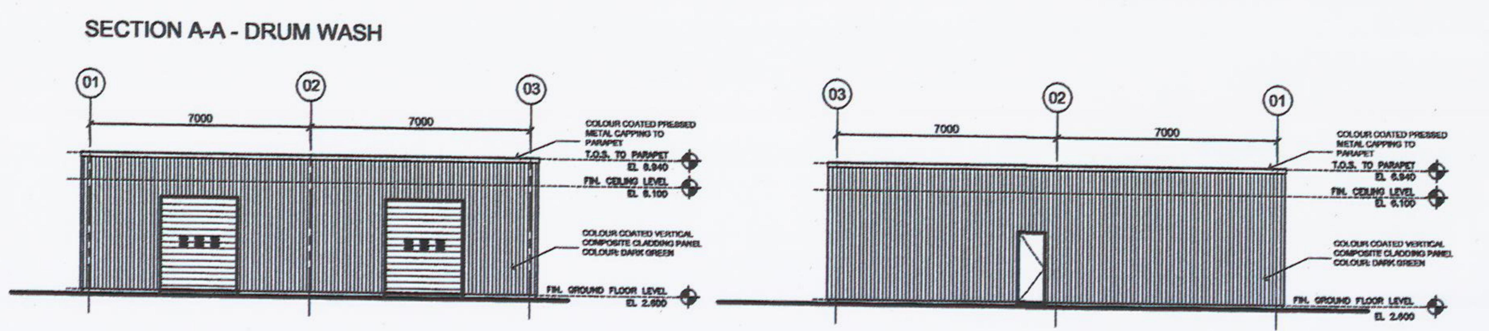
NORTH ELEVATION - DRUM WASH
