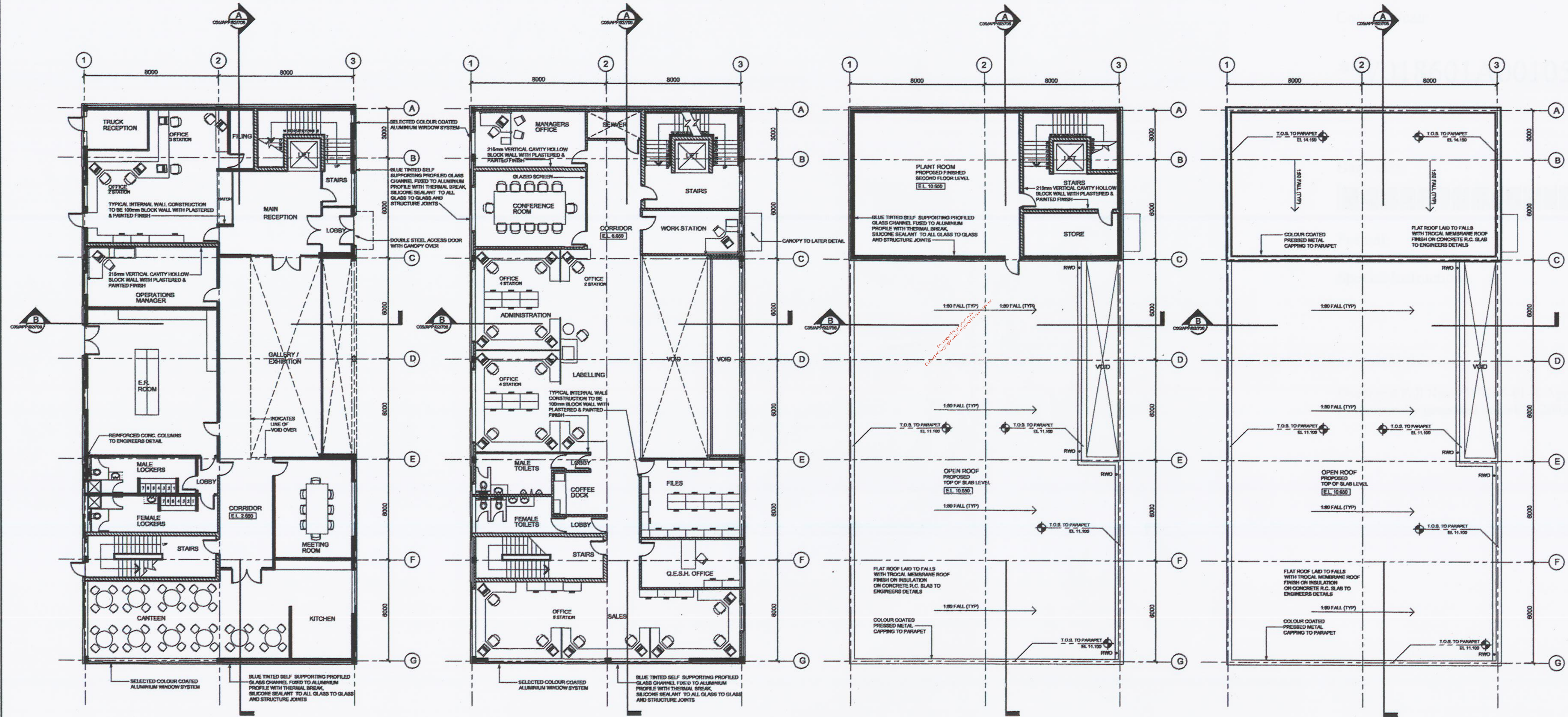
GROUND FLOOR - ADMINISTRATION BLOCK
