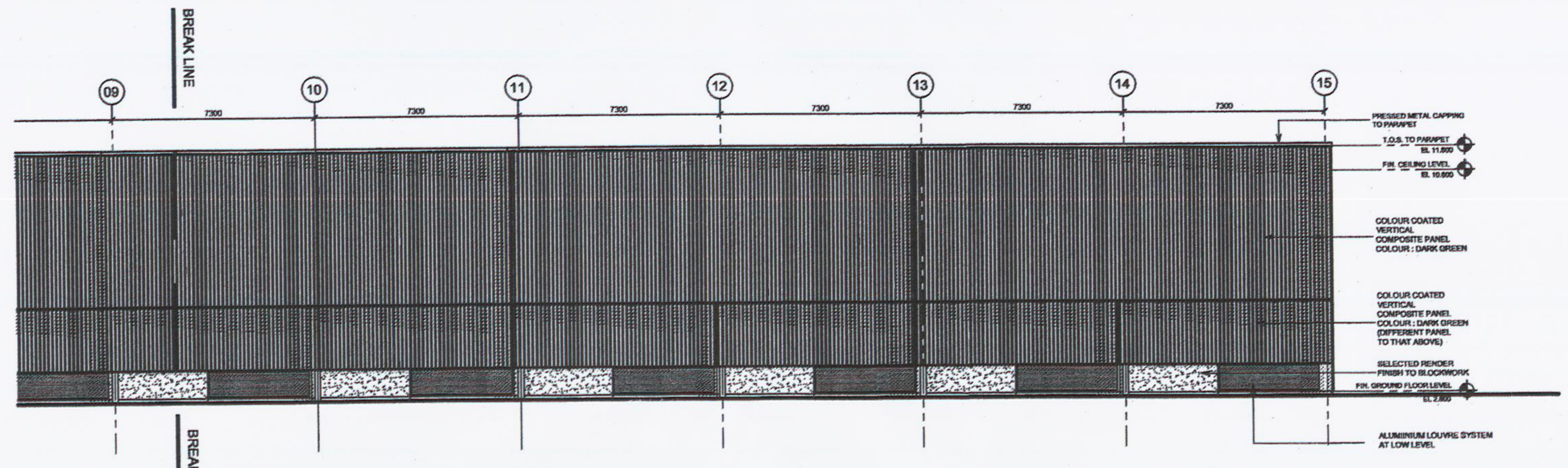
PART NORTH ELEVATION- TRANSFER STATION SCALE: 1-100
