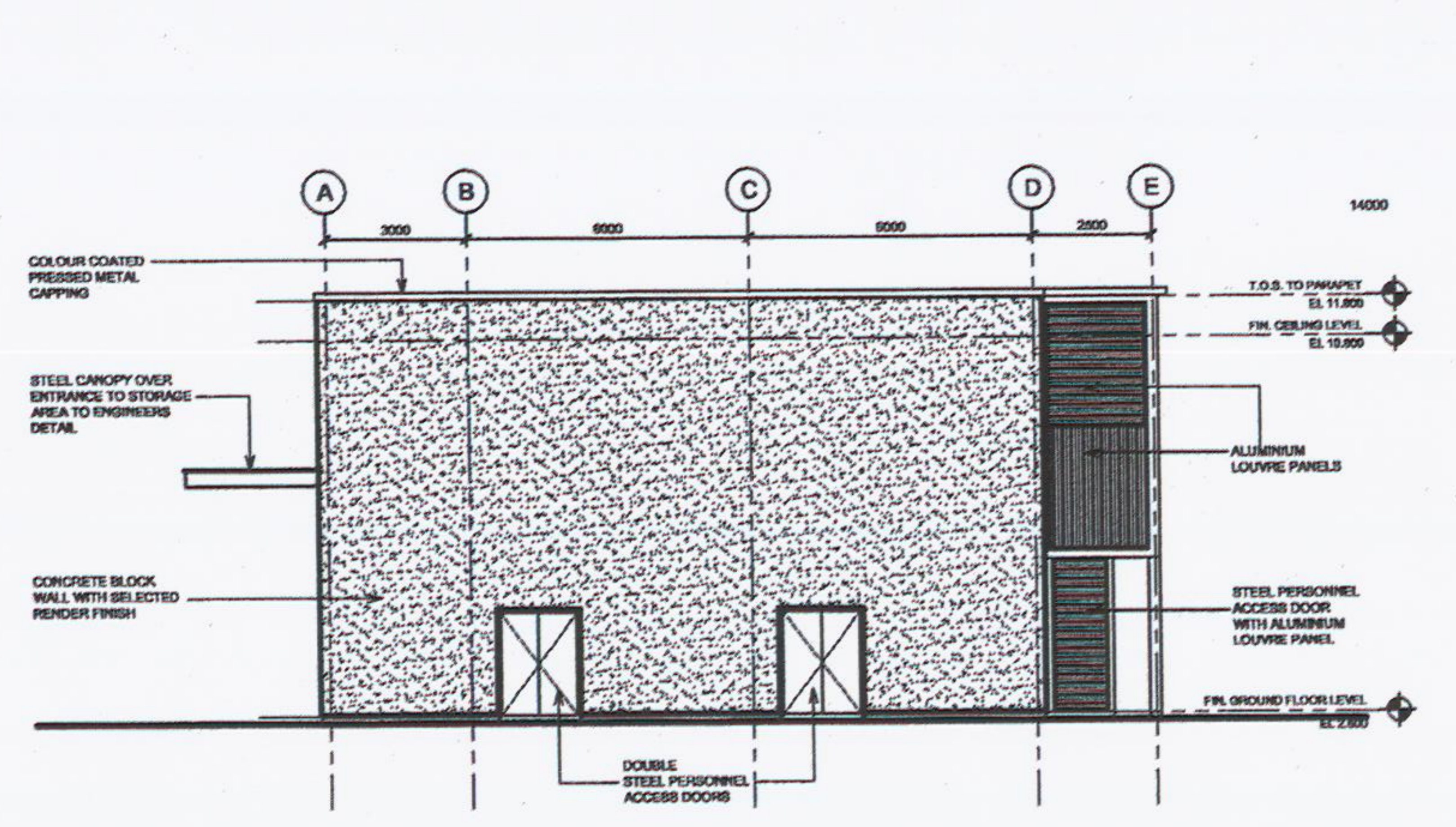
EAST ELEVATION - TRANSFER STATION SCALE: 1-100
