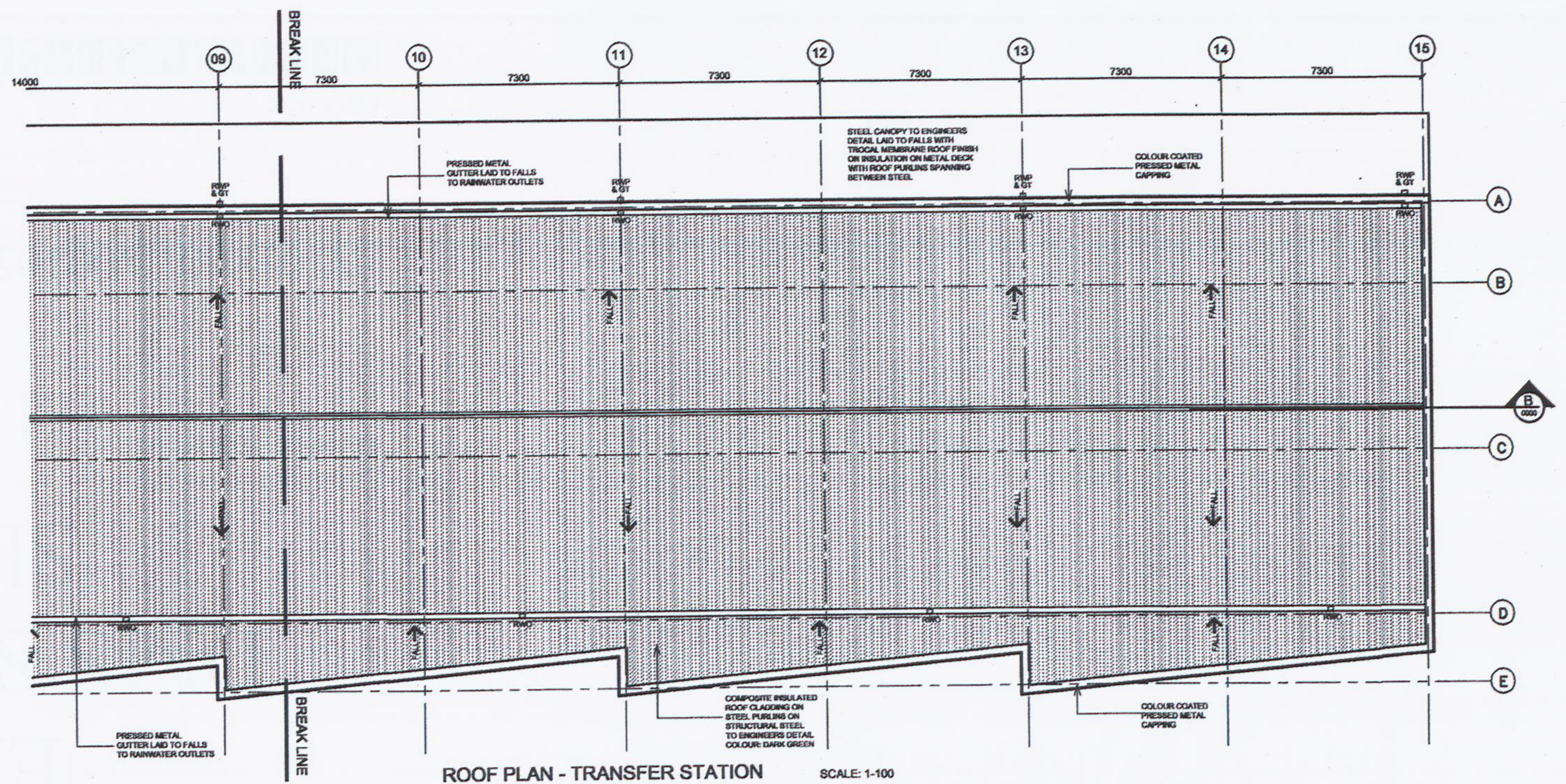
ROOF PLAN - TRANSFER STATION SCALE: 1:100
