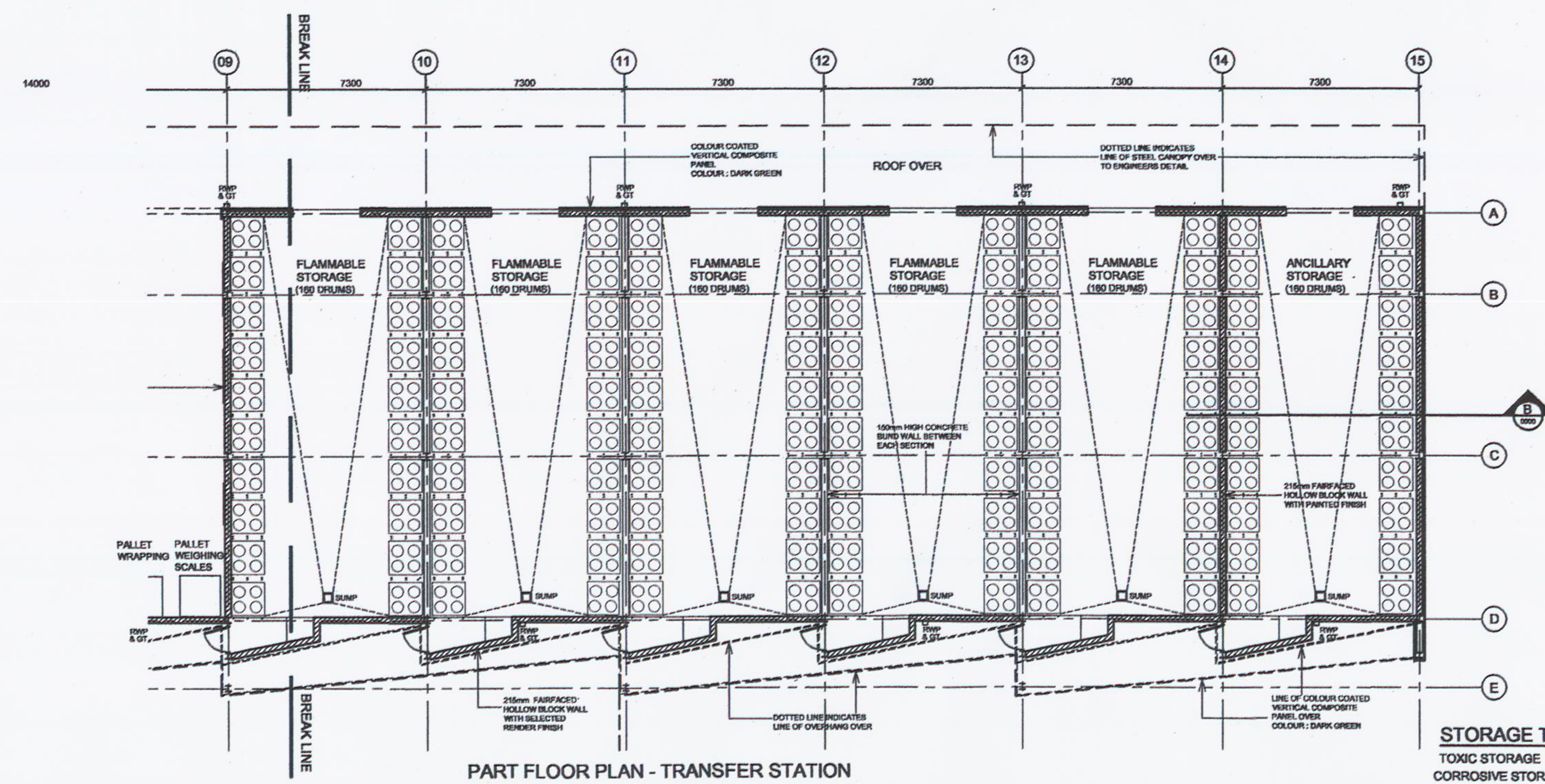
PART FLOOR PLAN - TRANSFER STATION SCALE: 1:100
