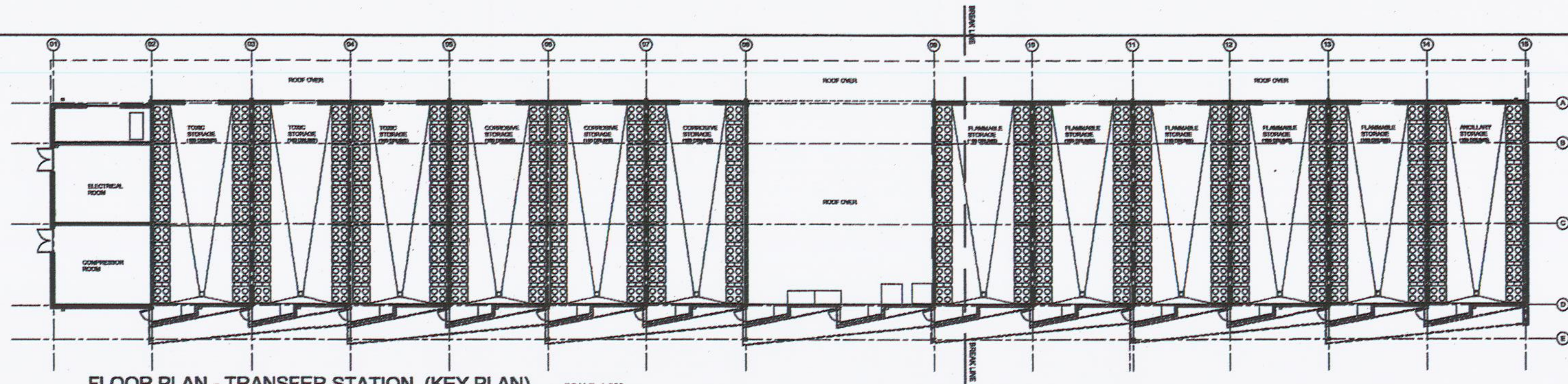
FLOOR PLAN - TRANSFER STATION (KEY PLAN) SCALE: 1:200
