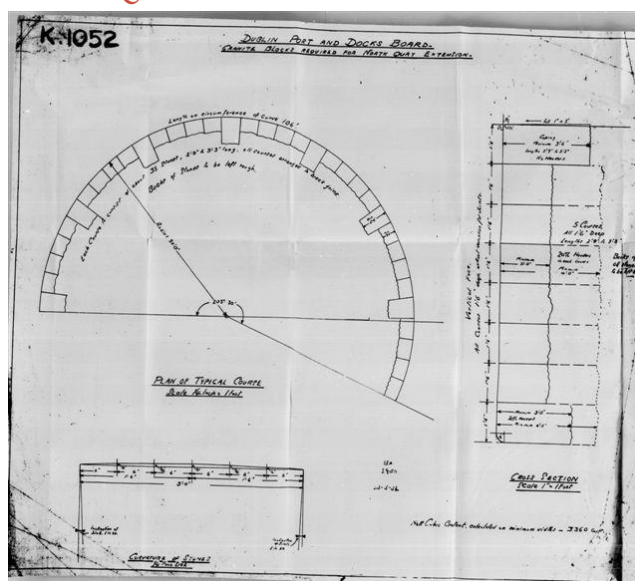
PLATE 7 SHOWING LAYOUT OF CURVED GRANITE BLOCKS (c 1938)
