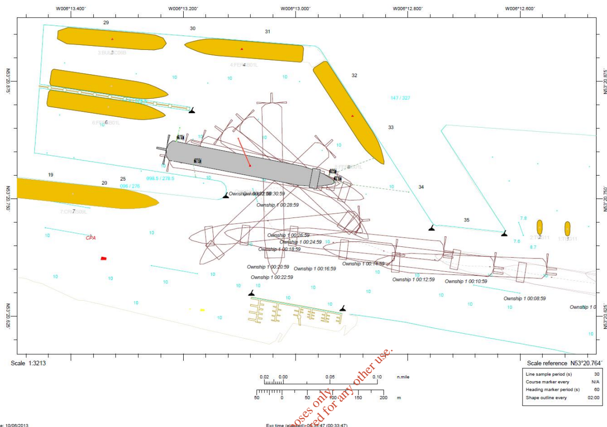
FIGURE 4 SAMPLE OUTPUT FROM THE NAVIGATION SIMULATION STUDY
