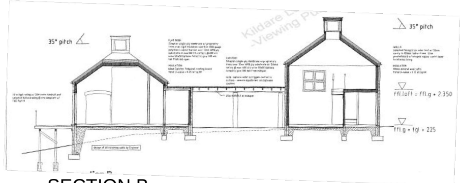
SECTION B
