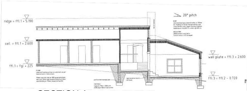
SECTION A
