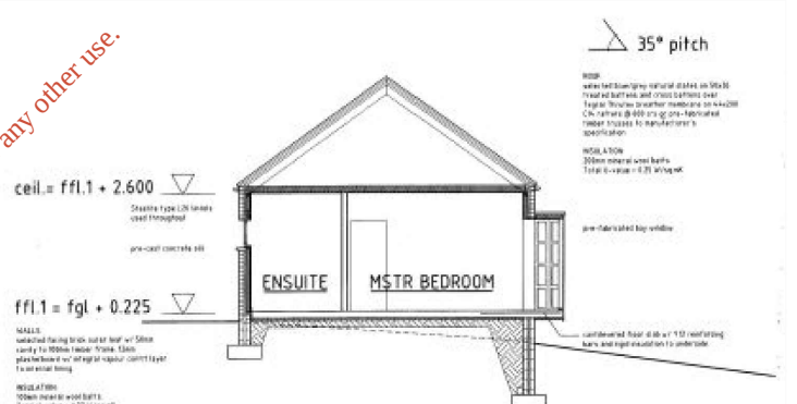
SECTION C
