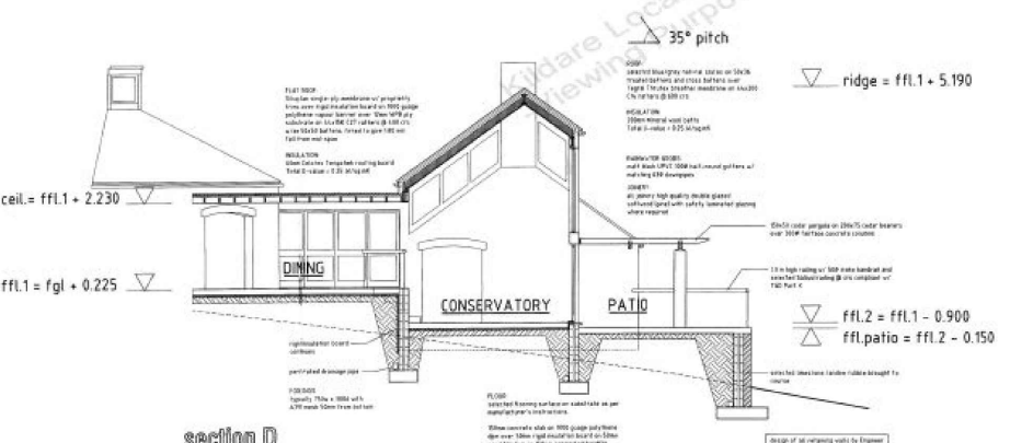
SECTION D
