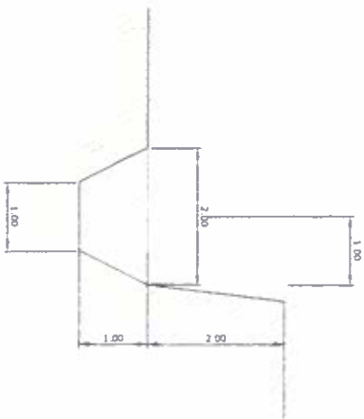
TYPICAL DETAIL THROUGH HIGH FIELD TOE DRAIN (A) AND DRAIN (B) (Refer to Draw No. CDR-11-PD-011) SCALE 1:50
