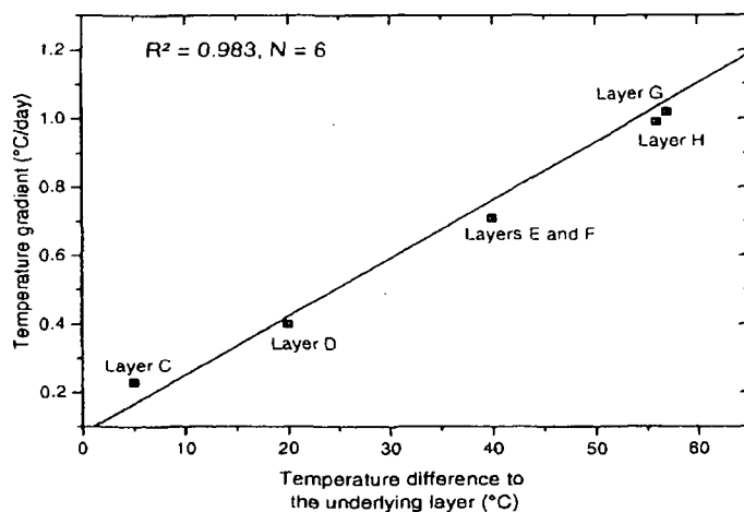
Fig. 6. Calculated gradient of temperature increase of the different layers vs. the temperature of the underlying layer in time of depositing the next one (shown is the regression line).
