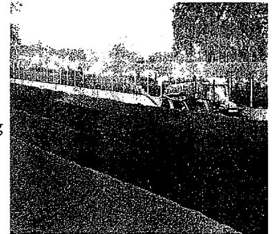
Rain-off and storm waters being re-applied back on to compost windrows at Organic Gold's yard.
